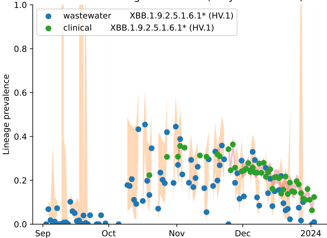
California Lineage Prevalence (daily unsmoothed)
