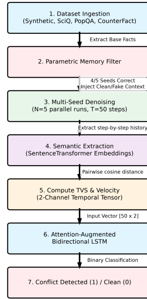
End-to-End Evaluation Pipeline for Knowledge Friction
