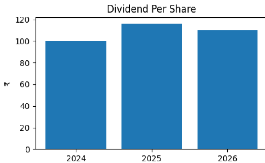
Figure 3: Dividend History
