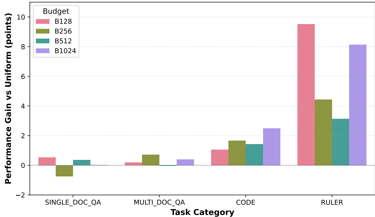
NAS Performance Gains by Task Type
