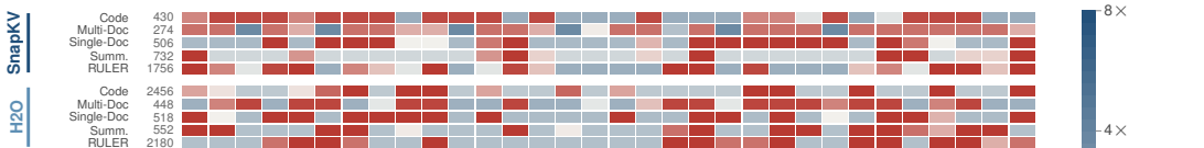
(b) MOSAIC's final configuration per cell (target budget; †: floor 16)
