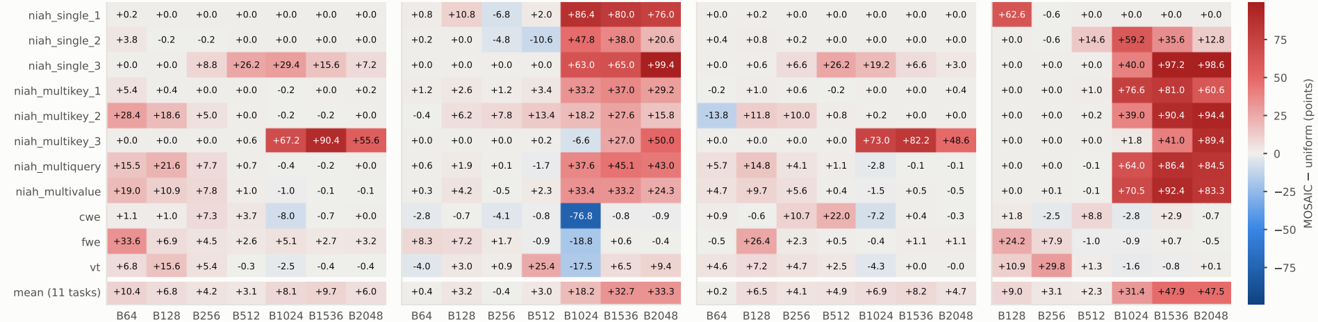
SnapKV
