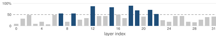
(c) Share of the allocations in (a) and (b) that give each layer more than its uniform share
