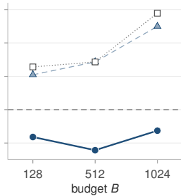
(b) SnapKV: Single-Doc QA shape on Code
