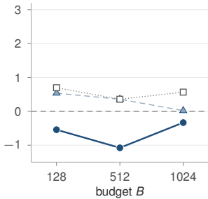
(a) SnapKV: Code shape on Single-Doc QA
