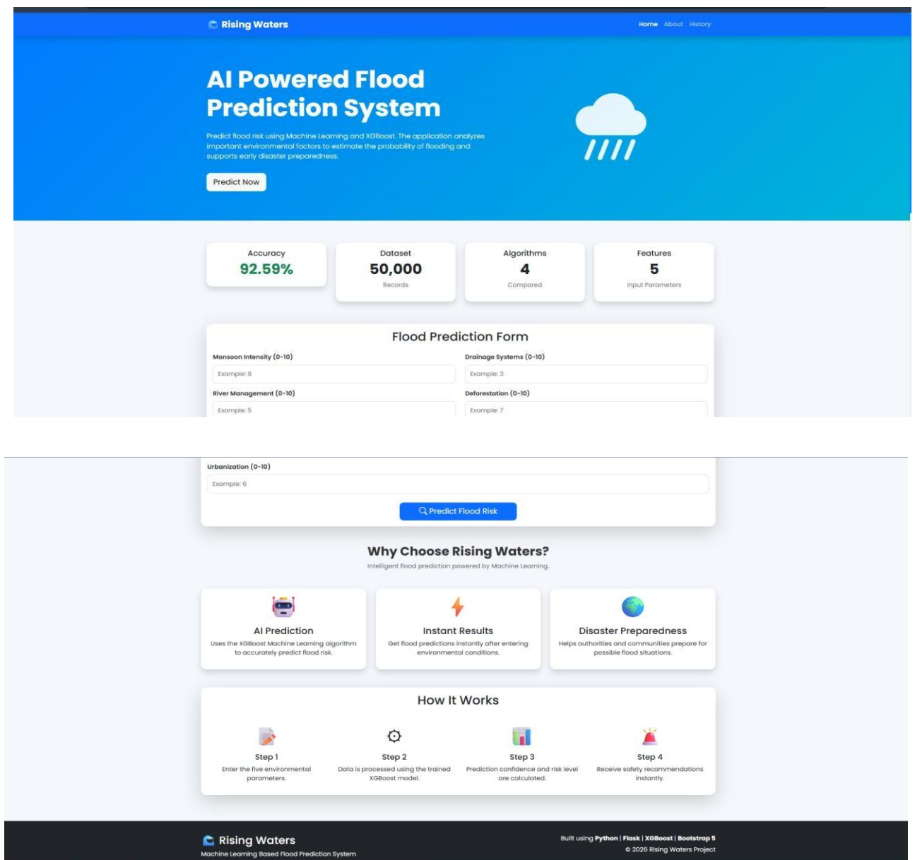
Figure 8.1 Home Page
