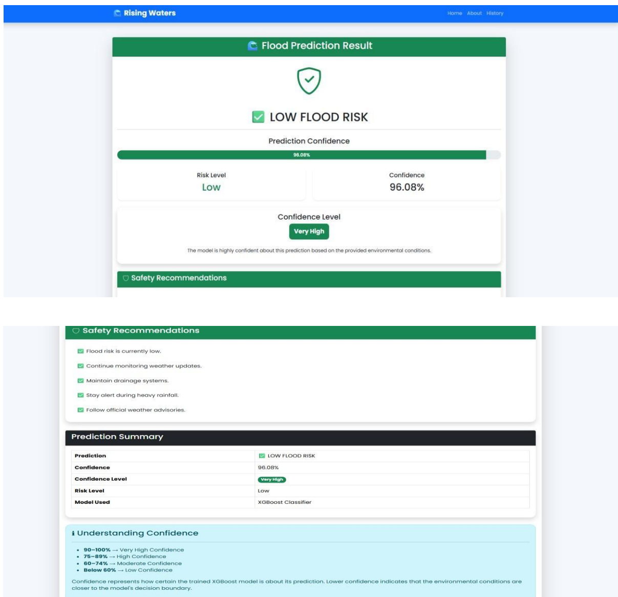
Figure 8.3 Prediction Result
