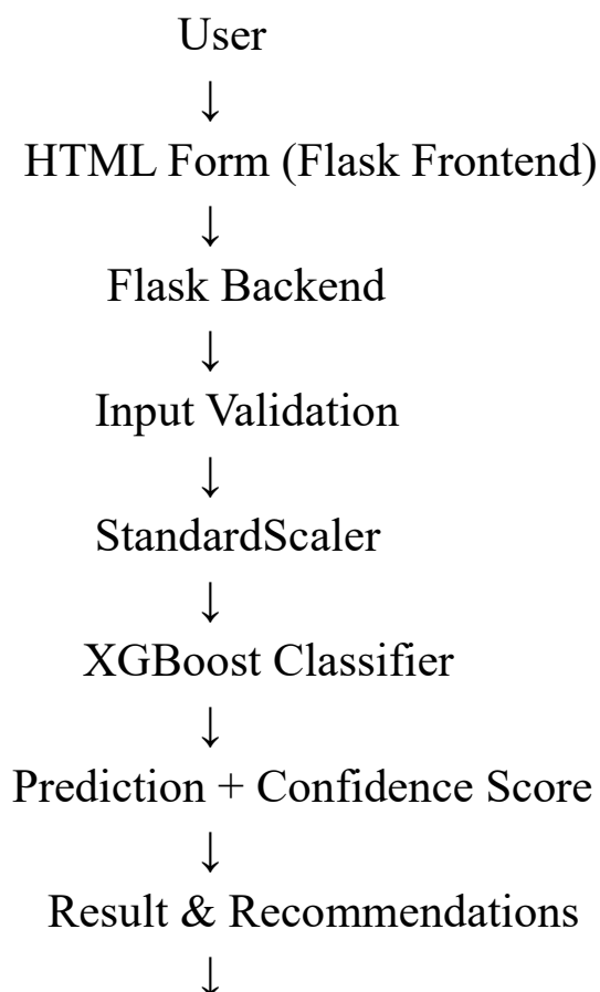
Figure 5.1.1 System Architecture
