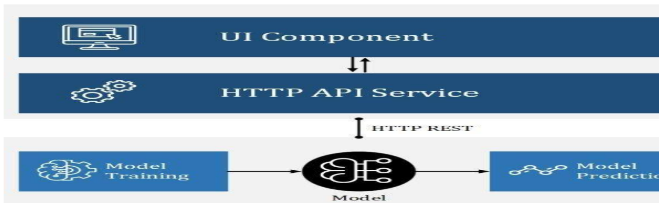
Figure 5.1.1 System Architecture
