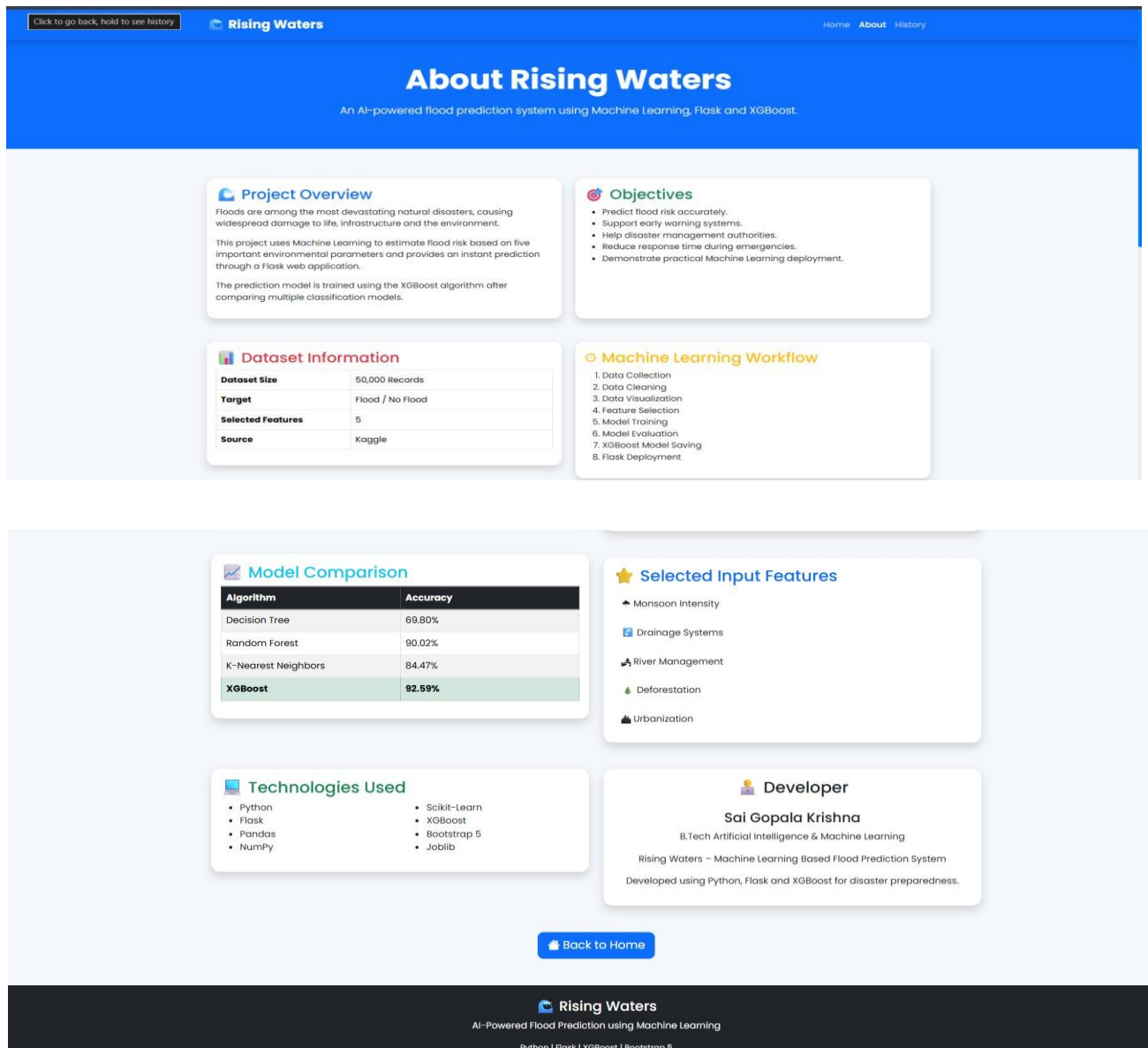
Figure 8.2 About Page
