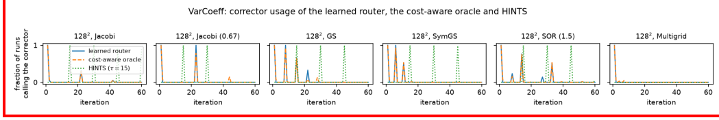
Figure 11: Variable-coefficient diffusion: corrector usage per iteration of the learned router, the cost-aware oracle and HINTS ( \tau=15 ) for every pairing (columns) and grid (rows).
