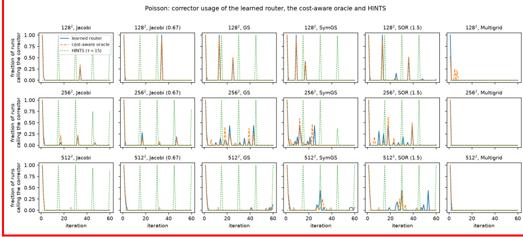
Figure 5: Poisson: fraction of test runs that execute a corrector call at each iteration, for the learned router, the cost-aware oracle and HINTS ( \tau=15 ), for every pairing (columns) and grid (rows; all test instances of each grid).
