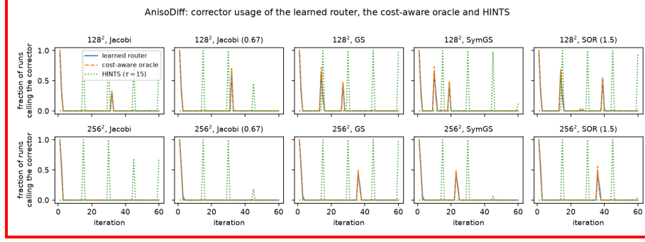
Figure 9: Anisotropic diffusion: corrector usage per iteration of the learned router, the cost-aware oracle and HINTS ( \tau=15 ) for every pairing (columns) and grid (rows).
