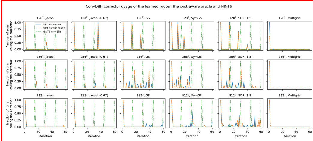
Figure 7: Convection–diffusion: corrector usage per iteration of the learned router, the cost-aware oracle and HINTS ( \tau=15 ) for every pairing (columns) and grid (rows).
