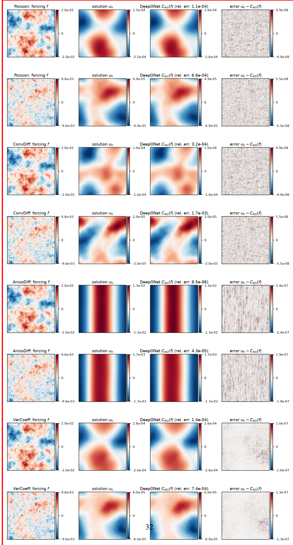
Figure 2: One-shot corrector predictions on the 128 \times 128 grid (two test instances per equation):
