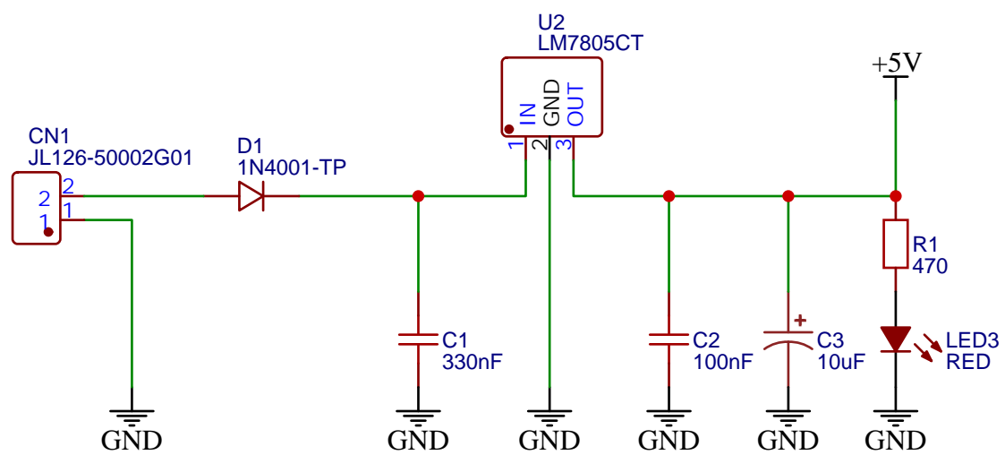
Power Supply
