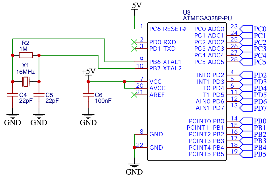
Controller
