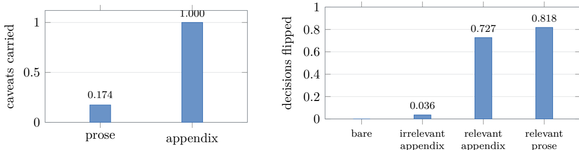
Figure 5: The out-of-band channel, both halves. Left : share of both-judge caveat sentences reaching the final artifact through writer prose against a mechanically assembled appendix (zero-generation design; byte-identical prose in both arms). Right : share of registered two-token reader decisions flipped by a planted decision-relevant caveat, by delivery arm (11 items, 440 reads; the irrelevant-appendix arm carries a matched caveat that does not bear on the decision). Uptake is content-specific (+0.691 [+0.455, +0.891] over the irrelevant control) and at parity with in-prose placement (+0.091 [-0.036, +0.218]).
