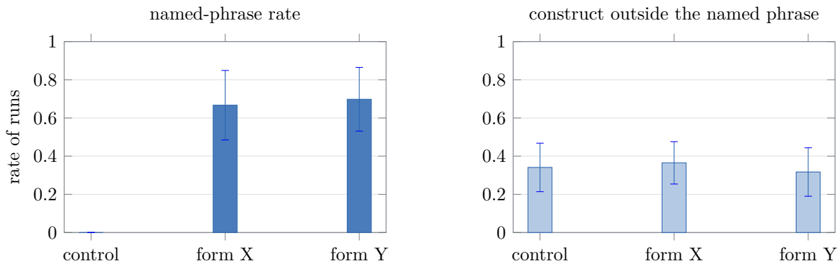
Figure 1: The phrase-swap experiment (378 runs, cluster-bootstrap 95% CIs over 18 cases). Left: each instructed arm produces its own named phrase in about two thirds of runs; control never produces either, and cross-form leakage is 0/252. Right: the validated-judge construct rate outside the named phrase is statistically indistinguishable across all three arms. The instruction’s entire measurable effect is the phrase it names.
