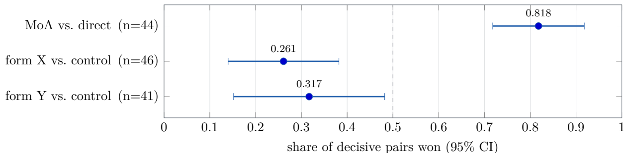
Figure 2: The preference experiment (order-debiased; a pair is decisive only when the same side wins both orderings; cluster-bootstrap CIs over cases). The aggregated pipeline beats the matched-length direct baseline decisively; both phrase-instructed arms lose to their own control, in counterbalanced forms whose only difference from control is the phrase. The dashed line is indifference.
