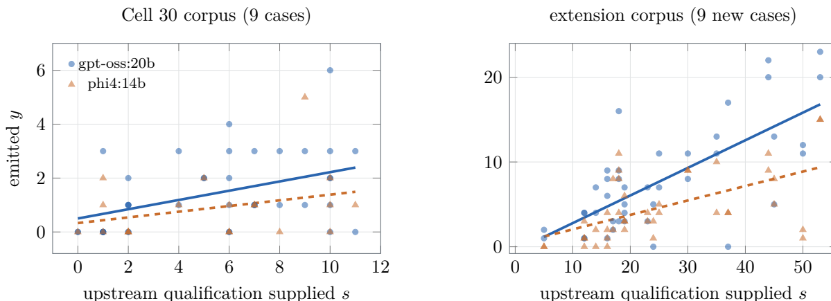
Figure 4: The transport coefficient y = ws + c , 144 runs over 18 cases and two writers. Each point is one run: upstream epistemic qualification supplied by the seats against qualification emitted by the writer, both counted by the validated two-judge sentence protocol. Lines are within-panel least-squares fits. The panels are separated because the two corpora occupy different supply regimes (mean s 5.4 against 25.3); pooling them produces a slope that is essentially the line between the two clusters, so no pooled fit is drawn. Within-panel slopes: gpt-oss 0.172 [+0.052, +0.297] and 0.326 [+0.207, +0.434]; phi4 0.105 [−0.031, +0.273] and 0.170 [+0.067, +0.265]. Three of the four exclude zero, and phi4’s right-hand fit is an independent replication on nine cases the original corpus never contained. The writer emits a small fraction of what it is given, and the fraction is a property of the writing step rather than of one model.
