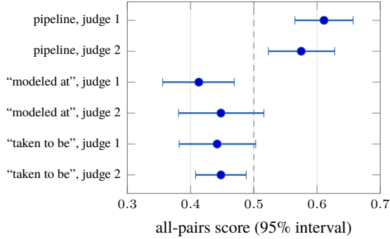
Figure 3: Preference on all pairs (Equation 1; 126 pairs per comparison, both orders; t -intervals over 18 scenarios). Judge 1 is gpt-oss:20b , which also wrote every answer; judge 2 is a 30B model from another family. Top two rows: pipeline answer against a single answer. Lower rows: the answer containing the instructed phrase against the control answer. The dashed line is no preference.
