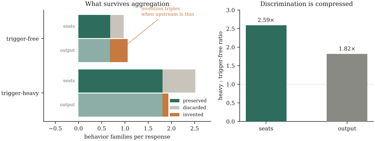
Figure 1: Left : for each condition, the upper bar is what the specialists raised, split into preserved and discarded; the lower bar is what the finished answer contains, split into traceable and invented. Right : the ratio between demanding and undemanding questions, as the specialists draw it and as it reaches the page. Means over 648 syntheses.
