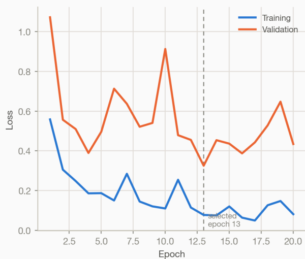
GoogLeNet - convergence generalization gap +0.087
