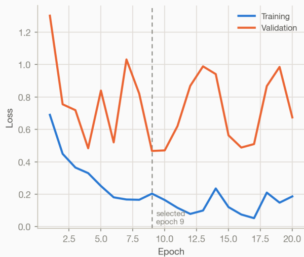
ResNet18 - convergence generalization gap +0.134
