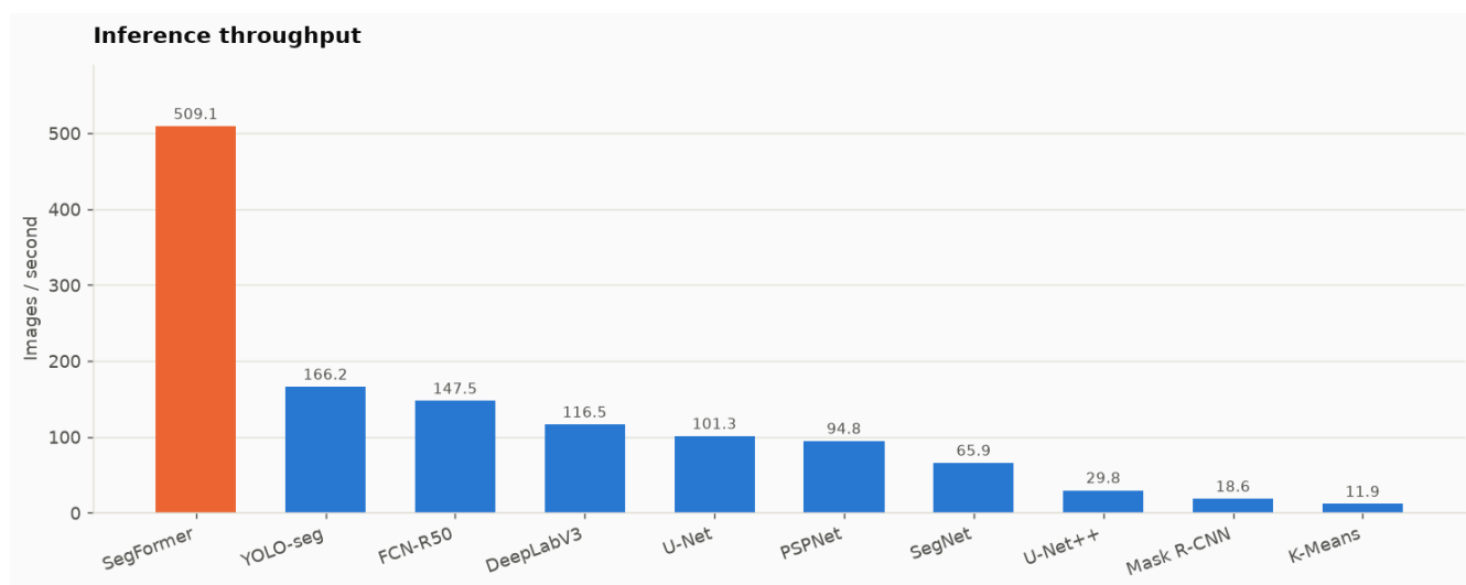
Inference throughput
