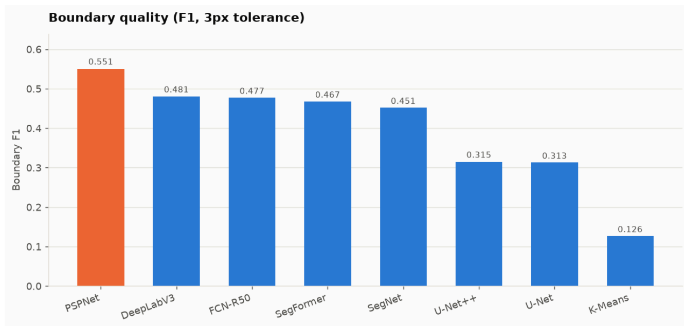
Boundary F1 at a 3-pixel tolerance
