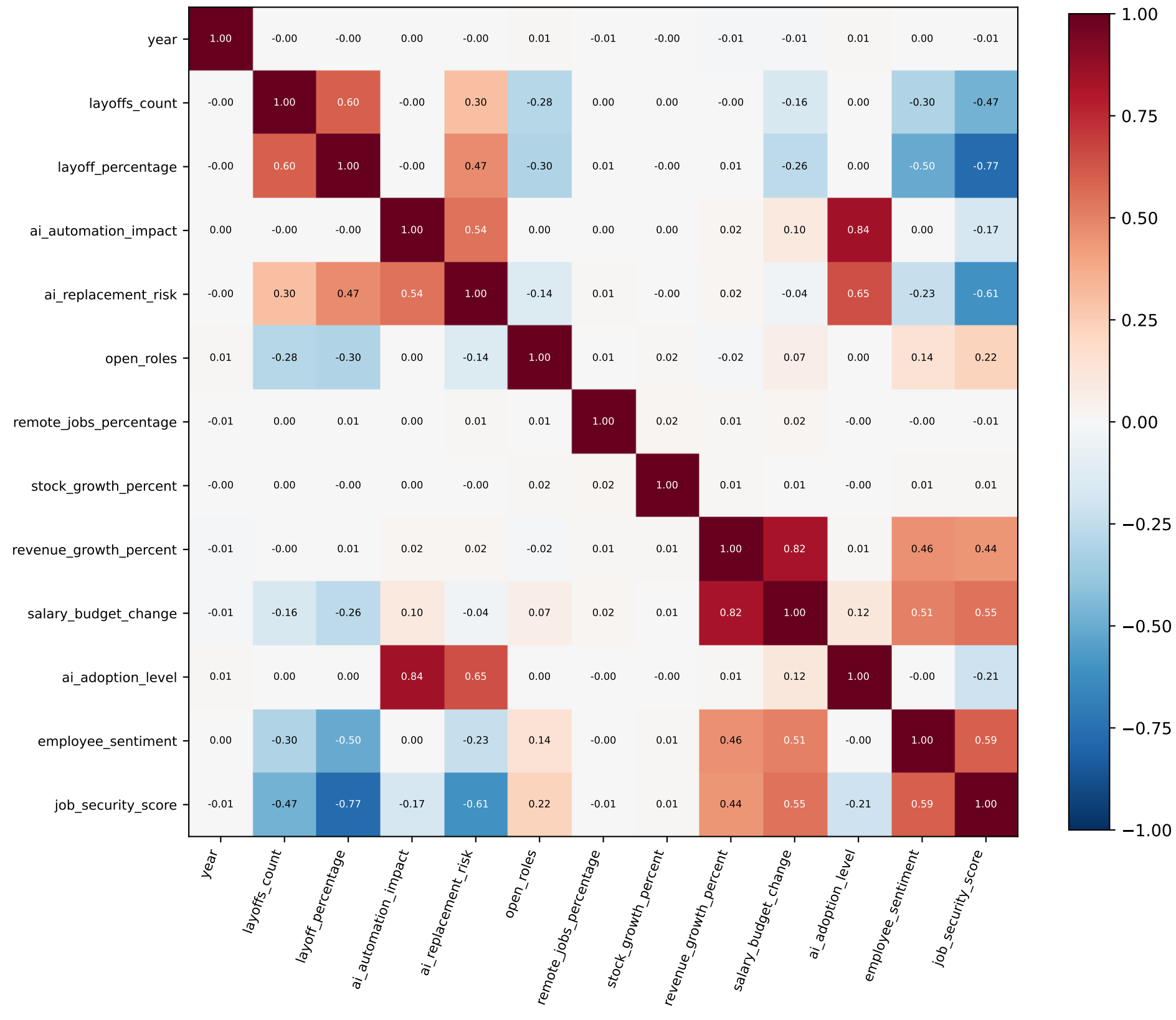
Correlation matrix of numeric features (n=12,000)
