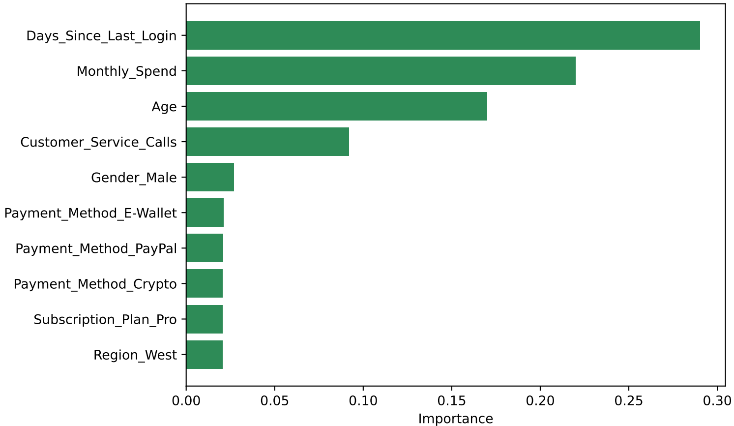
Random Forest: top 10 feature importances
