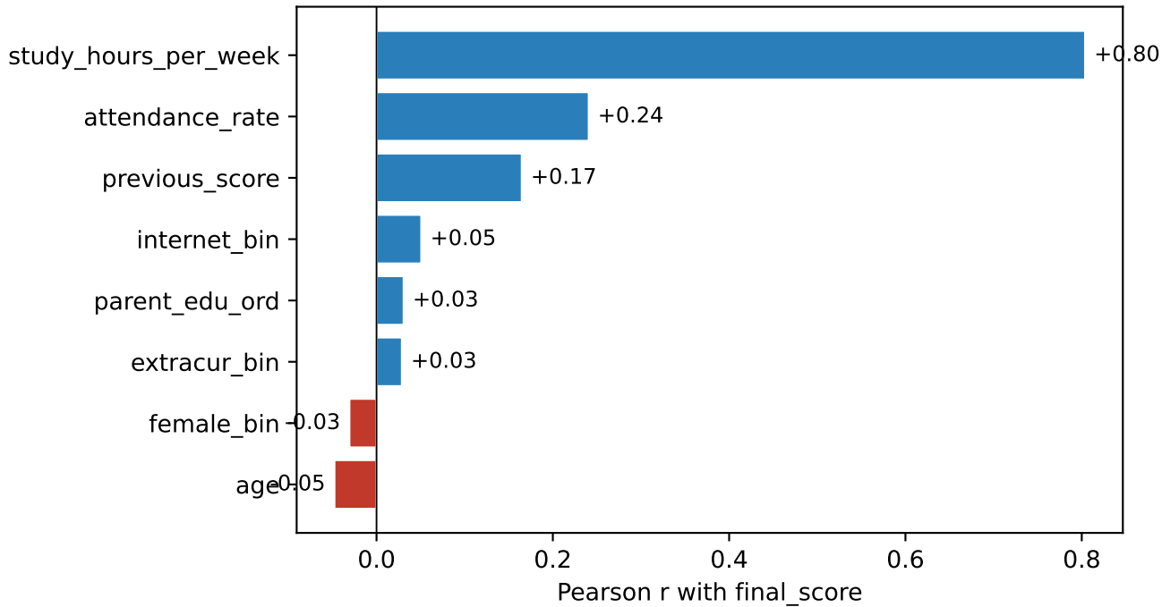
Figure 2. Correlation of predictors with final score
