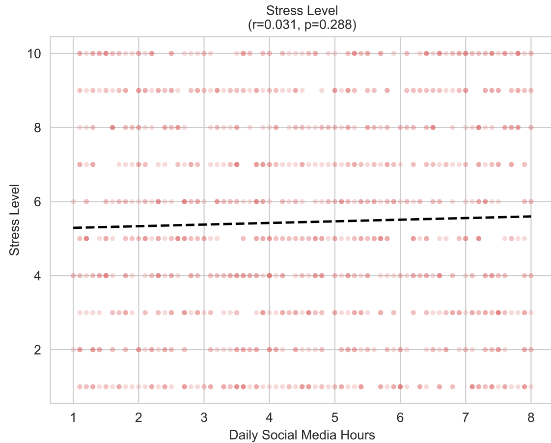
Figure 5: Social Media Hours vs Mental Health Outcomes
