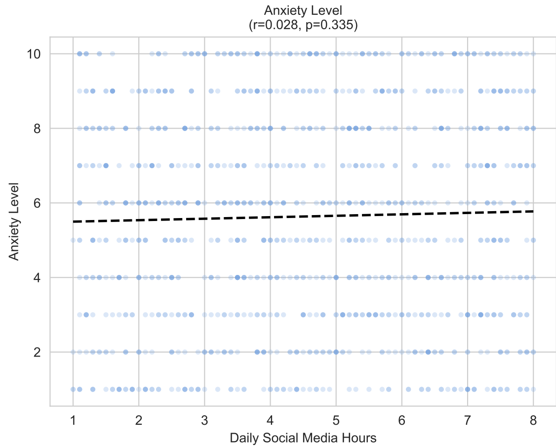
Figure 5: Social Media Hours vs Mental Health Outcomes
