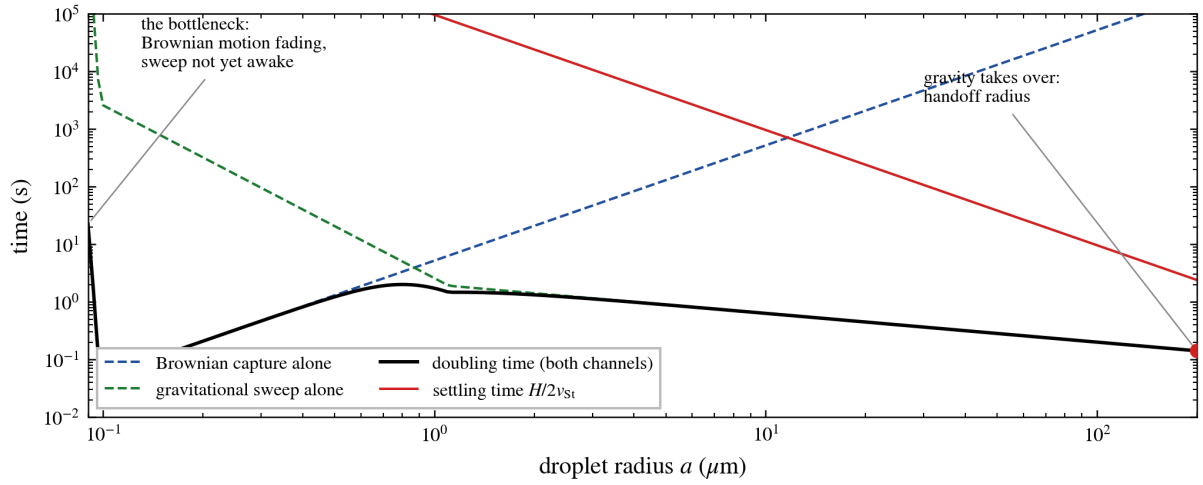
FIG. S6. Anatomy of the cascade clock. Per-doubling time versus droplet radius for the two transport channels and their sum (brine, 7.5 \text{ kV/cm} , central barrier), together with the settling time over half the cell depth. Brownian capture controls growth below a micron and gravitational sweep above it; the cascade's cost concentrates in the micron-scale bottleneck, and gravity takes over at the handoff radius.
