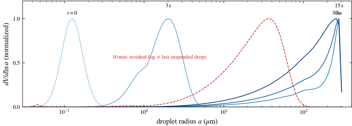
Figure 4: The coalescence cascade (population balance, 7.5 kV/cm, brine). Volume-weighted size distributions march through \sim 25 volume doublings within about thirty seconds (blue curves); by ten minutes (red dashed) the largest drops have settled out and the suspended remainder is the residual fog plus the last settling drops.
