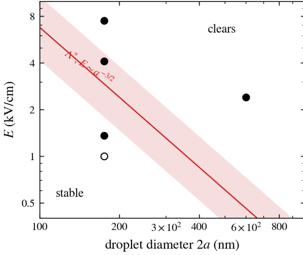
FIG. 2. The feasibility map. The \Lambda^* boundary ( E \sim a^{-3/2} ; orange band spans \Lambda^* = 0.3\text{--}2 ) in field-versus-size space, with operating points from Ref. [4]: filled, cleared; open, remained milky. The sweep’s cleared points bracket the boundary band, placing the operational threshold at the band’s lower edge; a 600 nm emulsion clears at modest fields because \Lambda \propto a^3 .
