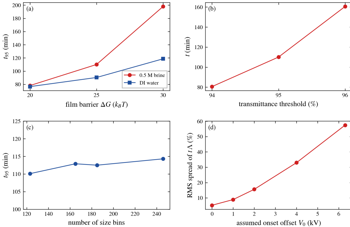
FIG. S1. Robustness of the headline numbers. (a) Sensitivity of the predicted optical clearing time to the film barrier over its 20–30 k_B T band, both water phases. (b) Stiffness of the operational endpoint: a one-percentage-point change in the transmittance threshold moves t_{95} by -27\%/+46\% . (c) Grid convergence of the population balance: doubling the size resolution shifts t_{95} by +3.8\% . (d) Onset-offset profile of the data collapse: the RMS spread of t \cdot \Lambda across the digitized sweep degrades monotonically with an assumed corona offset V_0 in the field reading, preferring V_0 = 0 .
