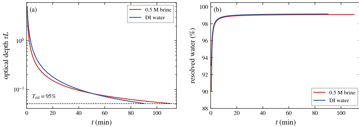
FIG. 5. Two clocks (population balance, 7.5 kV/cm). (a) The optical clock: droplet optical depth decays toward the 95%-transmittance threshold (dashed) in 90–110 min, brine (red) slower than DI water (blue). (b) The mass clock: resolved water exceeds 97% within minutes for both phases.
