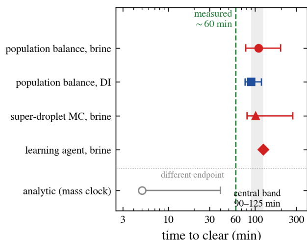
FIG. S2. Calibration-free predictions against the measured clearing time. Central estimates (symbols) and uncertainty ranges (bars) for the optical endpoint from the population balance (film-barrier band), the fixed-field super-droplet Monte Carlo (spread over 20 seeds), and the learning agent's value estimate, alongside the single measured batch value (dashed). The grey band is the range of central estimates quoted in the text. The analytic route (open symbol, below the rule) times the mass clock, a different observable, and is shown for completeness.
