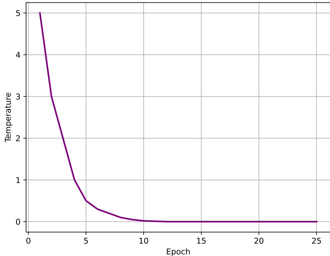
Quantization Temperature Schedule
