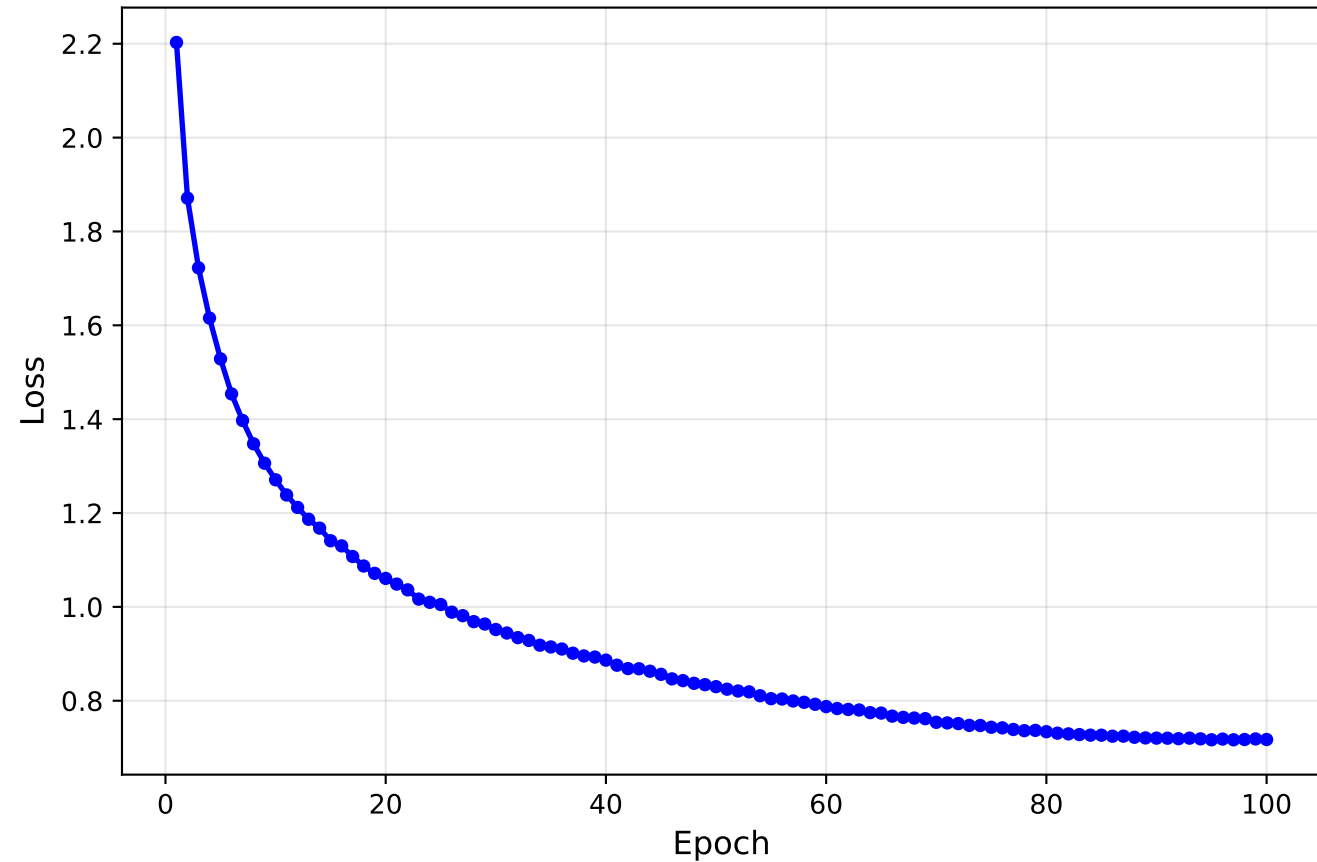
Training Loss
