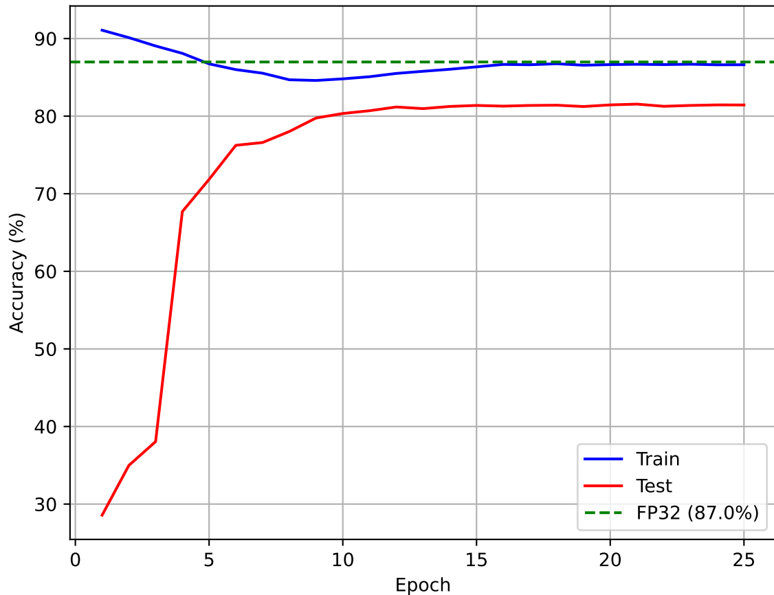
Progressive QAT Accuracy
