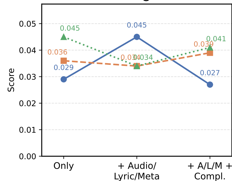
NDCG@20
