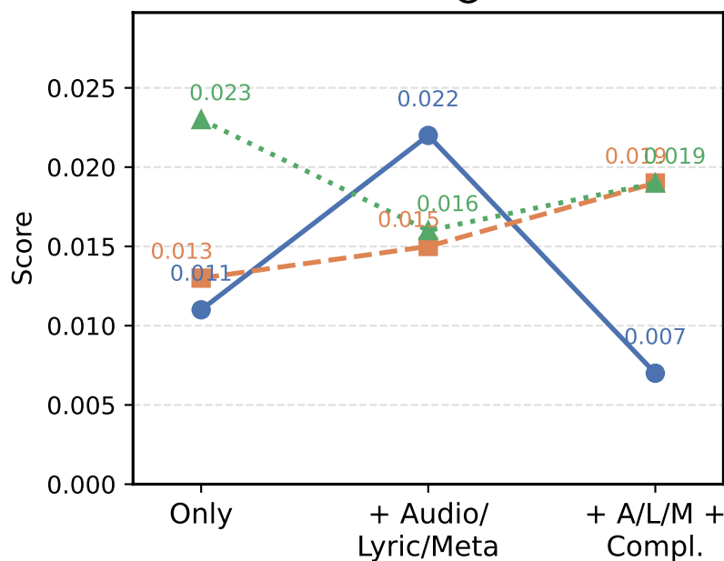
NDCG@5
