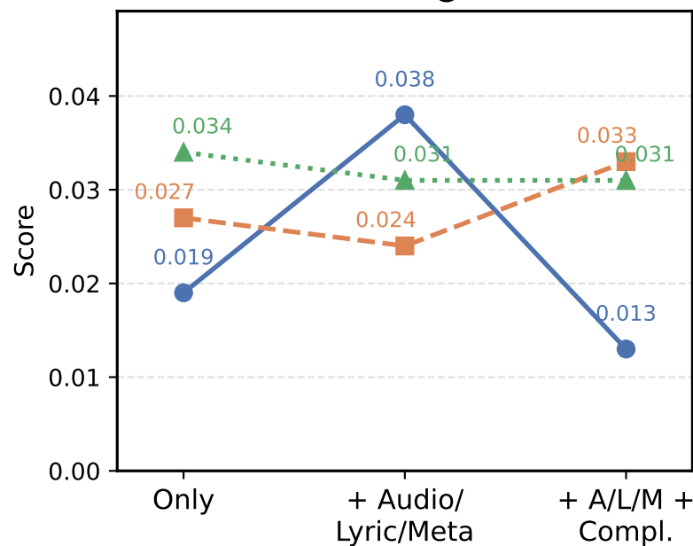
NDCG@5
