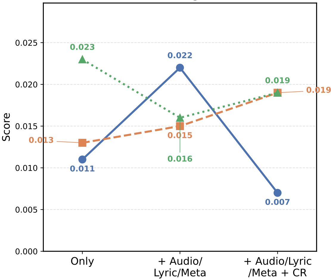
NDCG@5
