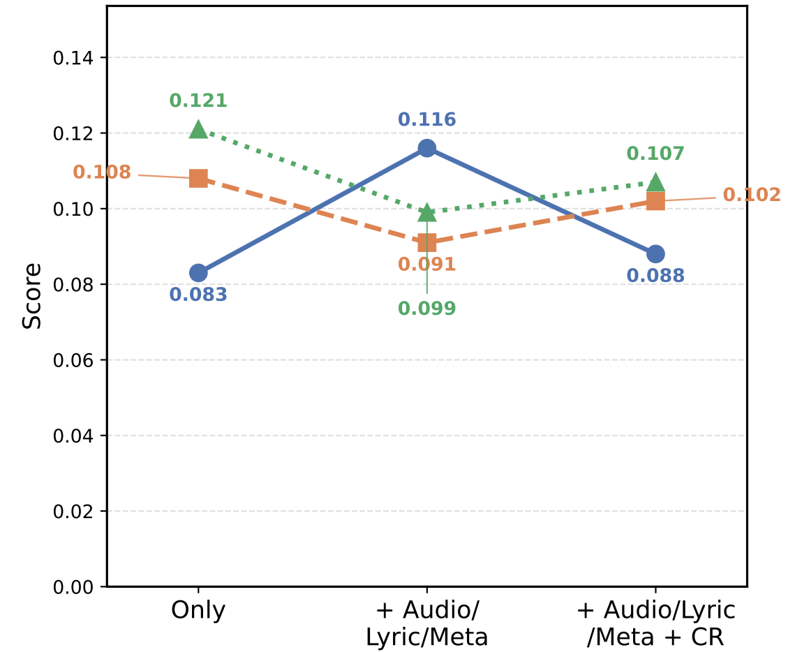
NDCG@20
