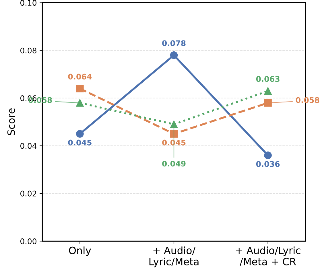
NDCG@10
