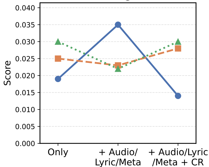
NDCG@10
