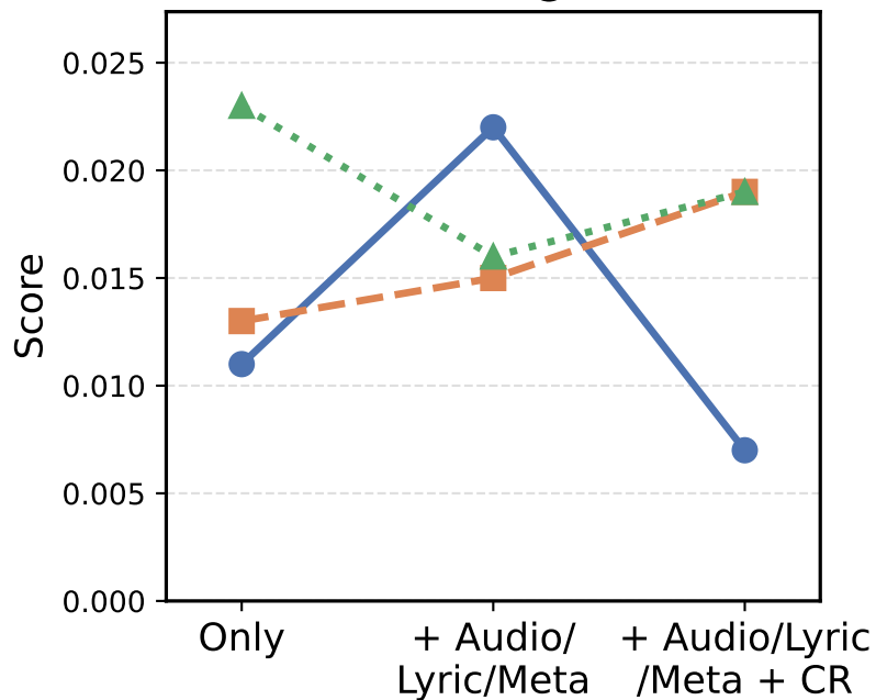
NDCG@5
