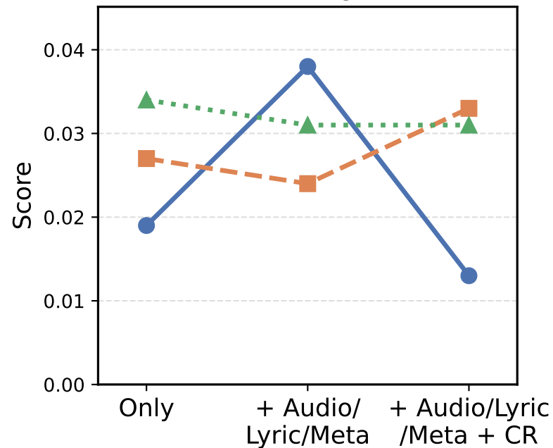
NDCG@5
