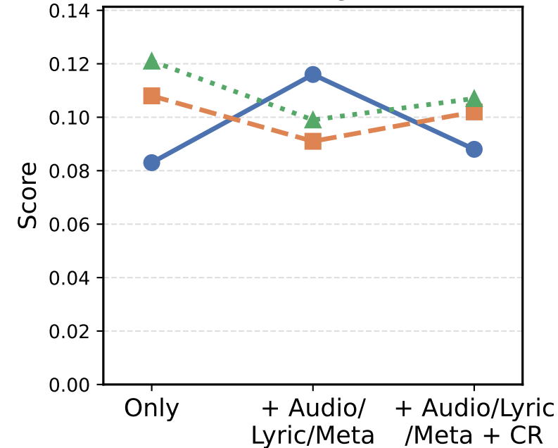
NDCG@20
