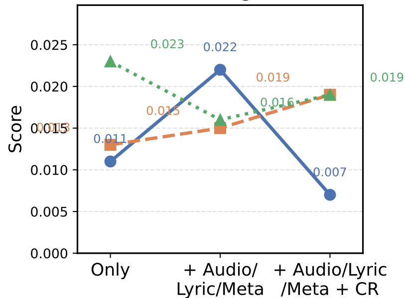
NDCG@5
