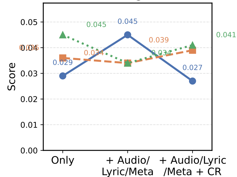
NDCG@20
