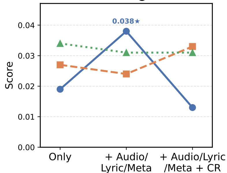
NDCG@5
