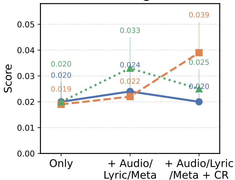
NDCG@5
