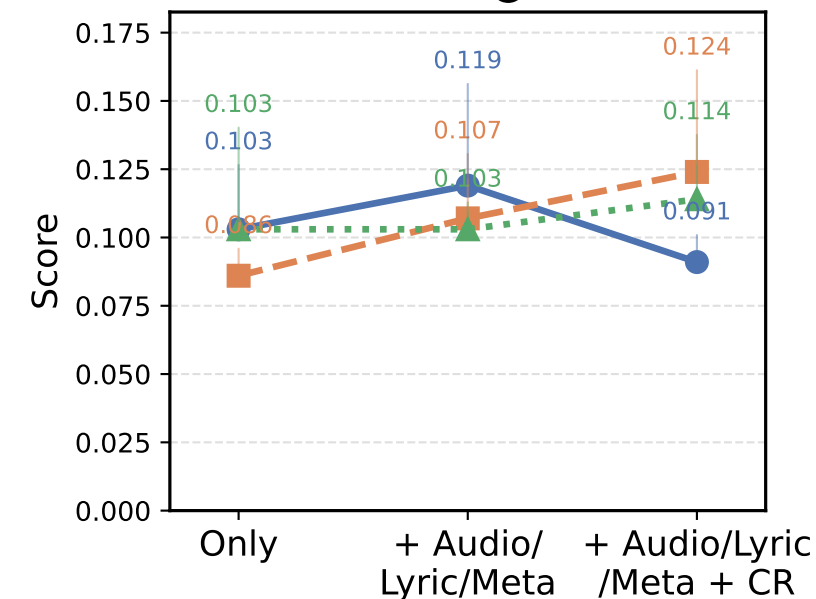
NDCG@20
