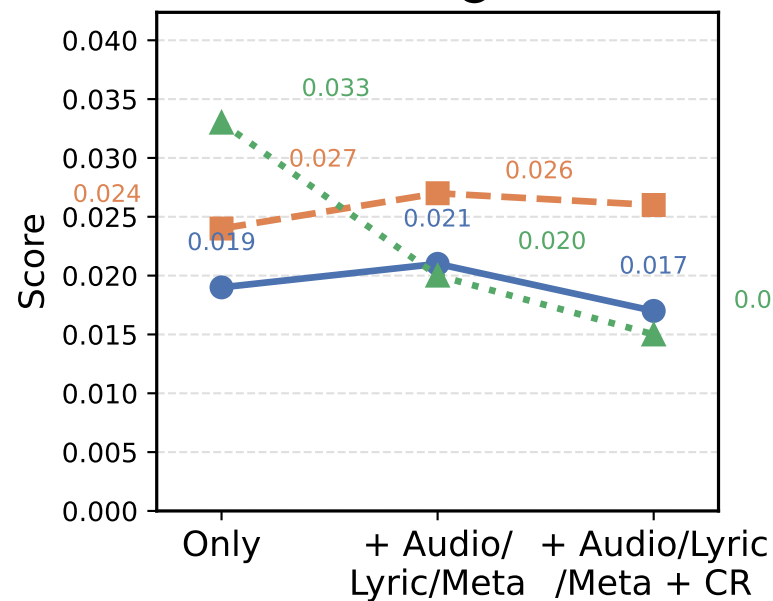
NDCG@10
