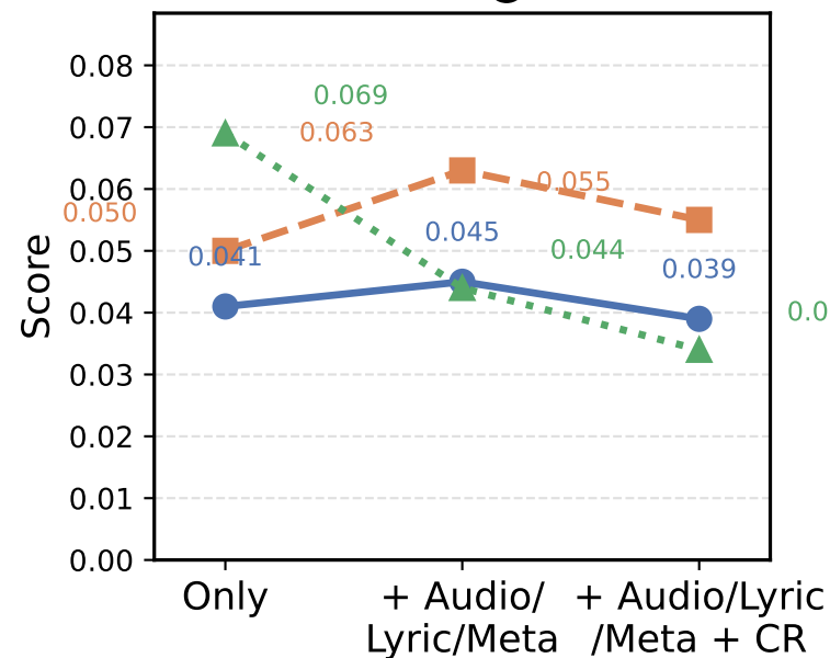
NDCG@10
