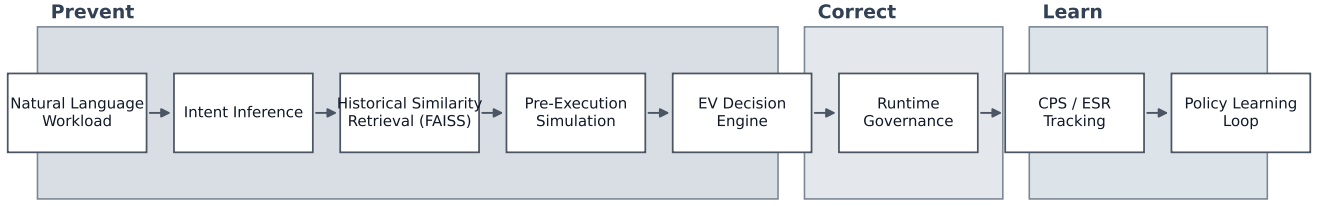
Figure 1: PBCP system architecture. The pipeline groups pre-billing prevention, runtime correction, and policy learning into one governance loop.
