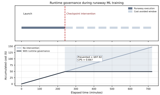
Figure 4: Runtime governance intervention during a runaway ML training workload. The intervention checkpoints prolonged execution at the anomaly boundary, preventing $97.92 of additional cost accumulation.
