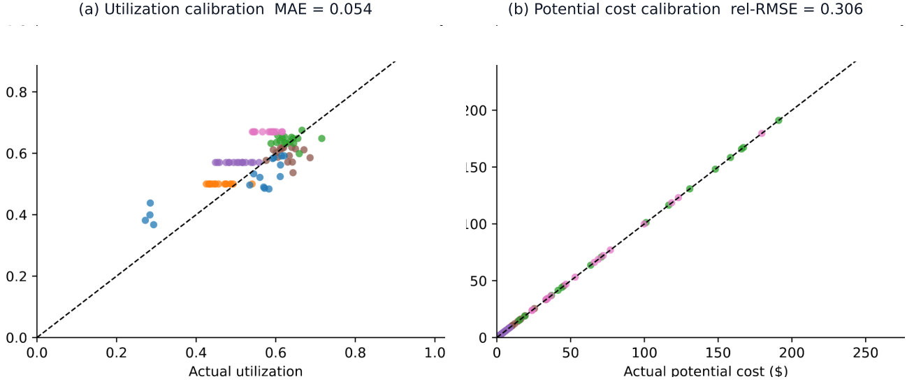
Figure 2: Simulation calibration for Exp 0. Predicted utilization closely tracks observed utilization, with utilization MAE of 0.054 and cost rel-RMSE of 0.306.
