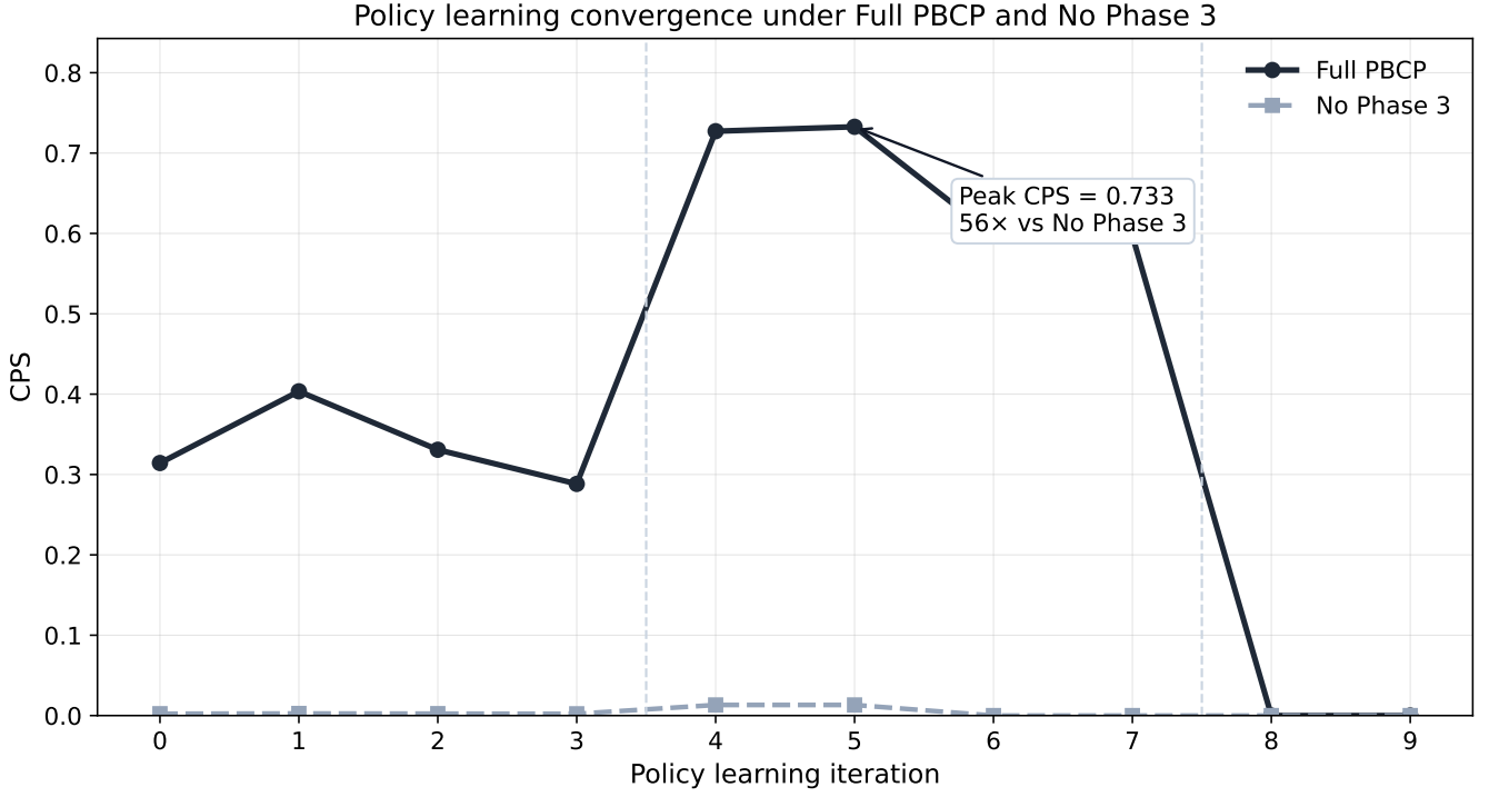
Figure 6: Policy-learning convergence in Exp 6. Full PBCP reaches peak CPS of 0.733 versus 0.013 for the No Phase 3 baseline, a 56 \times improvement.
