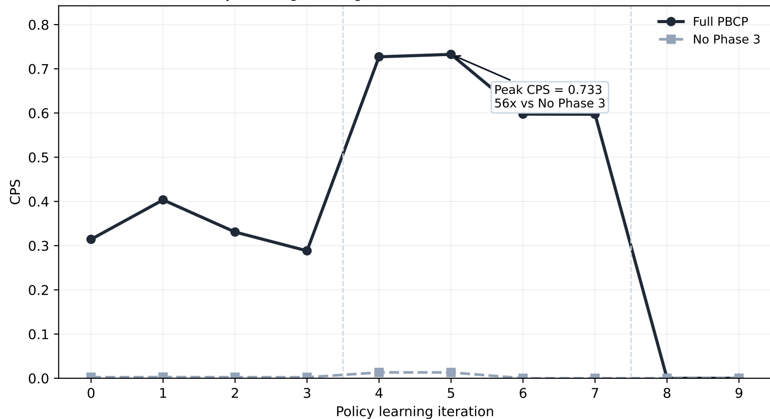
Policy learning convergence under Full PBCP and No Phase 3
