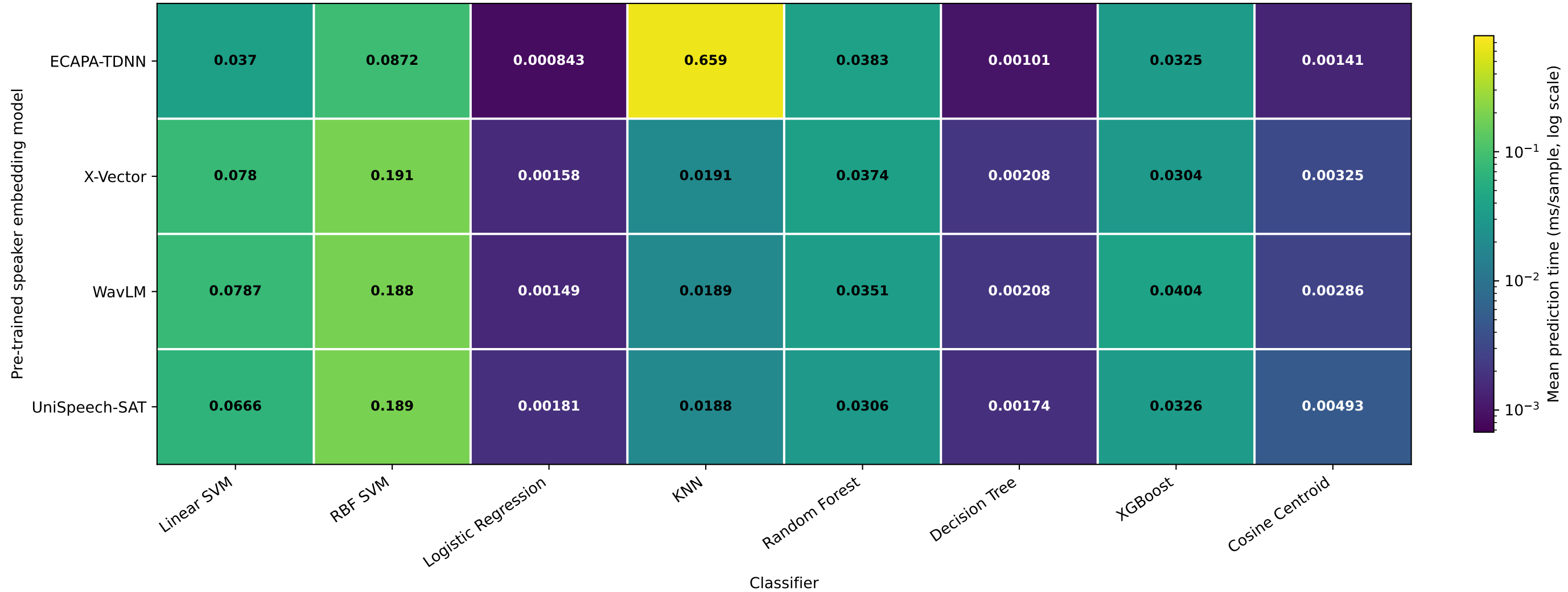
Classifier prediction latency by embedding model Strict chapter-held-out protocol
