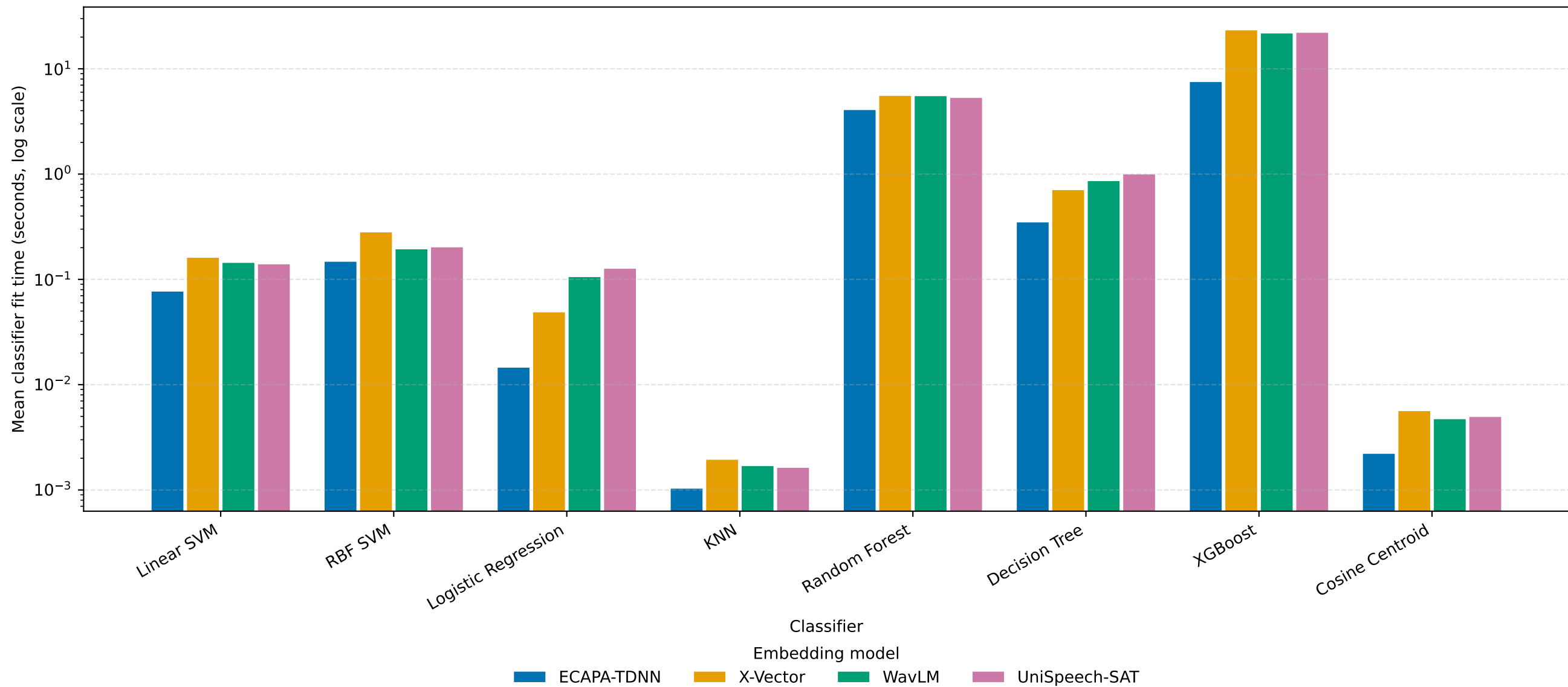
Classifier training-time comparison Strict chapter-held-out protocol
