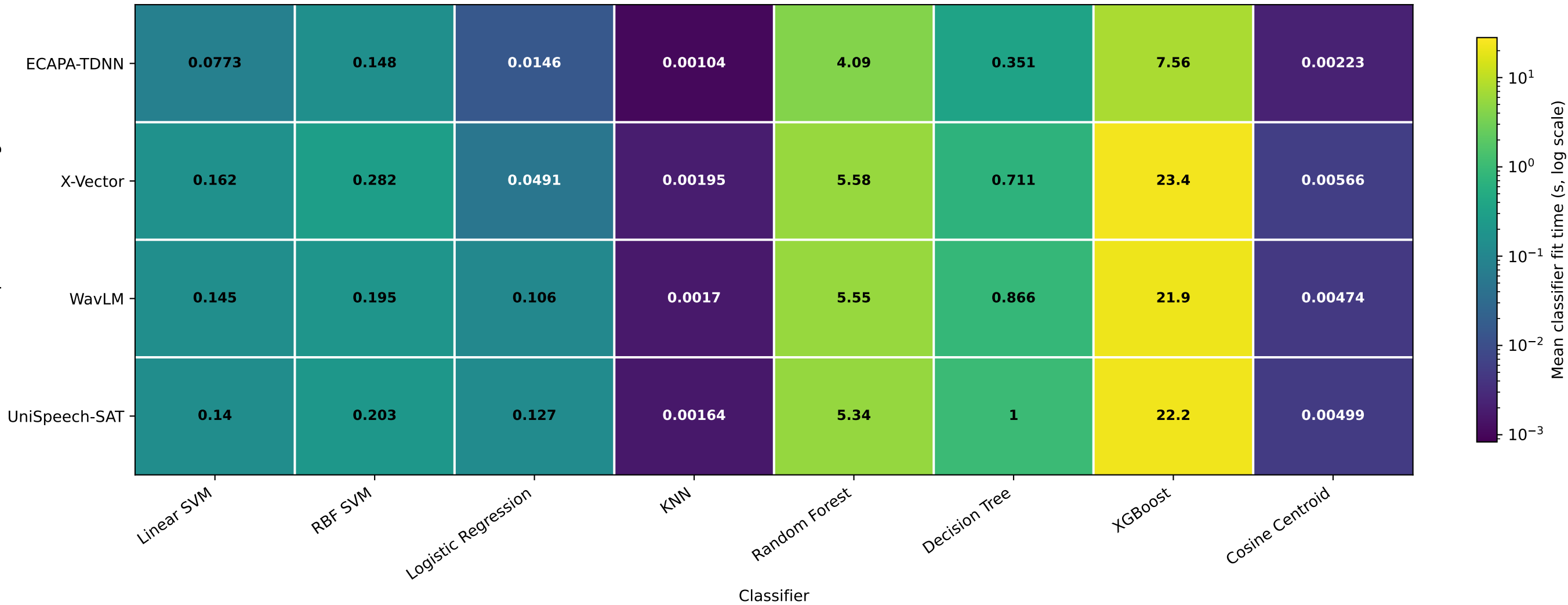
Classifier training time by embedding model Strict chapter-held-out protocol
