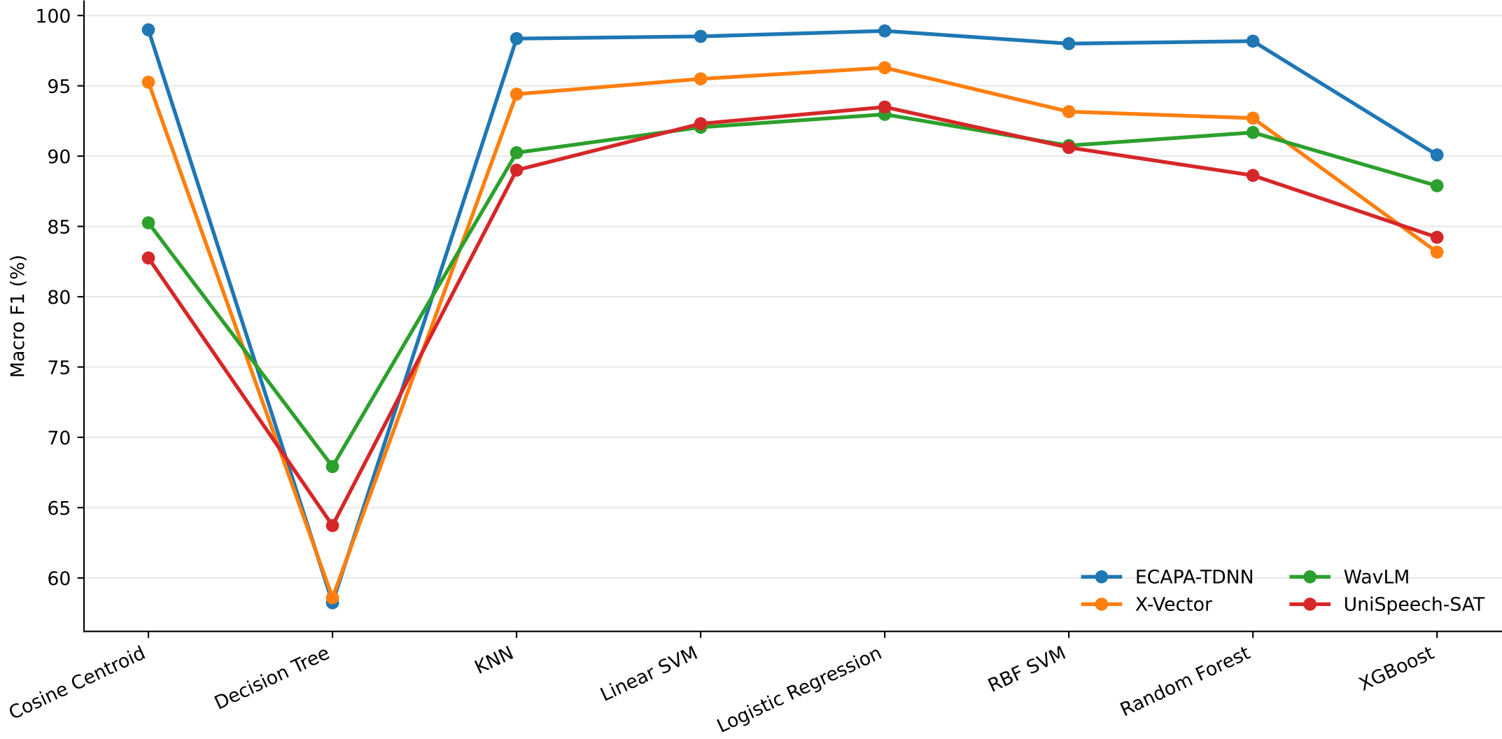
Macro F1 by Embedding Model and Classifier
