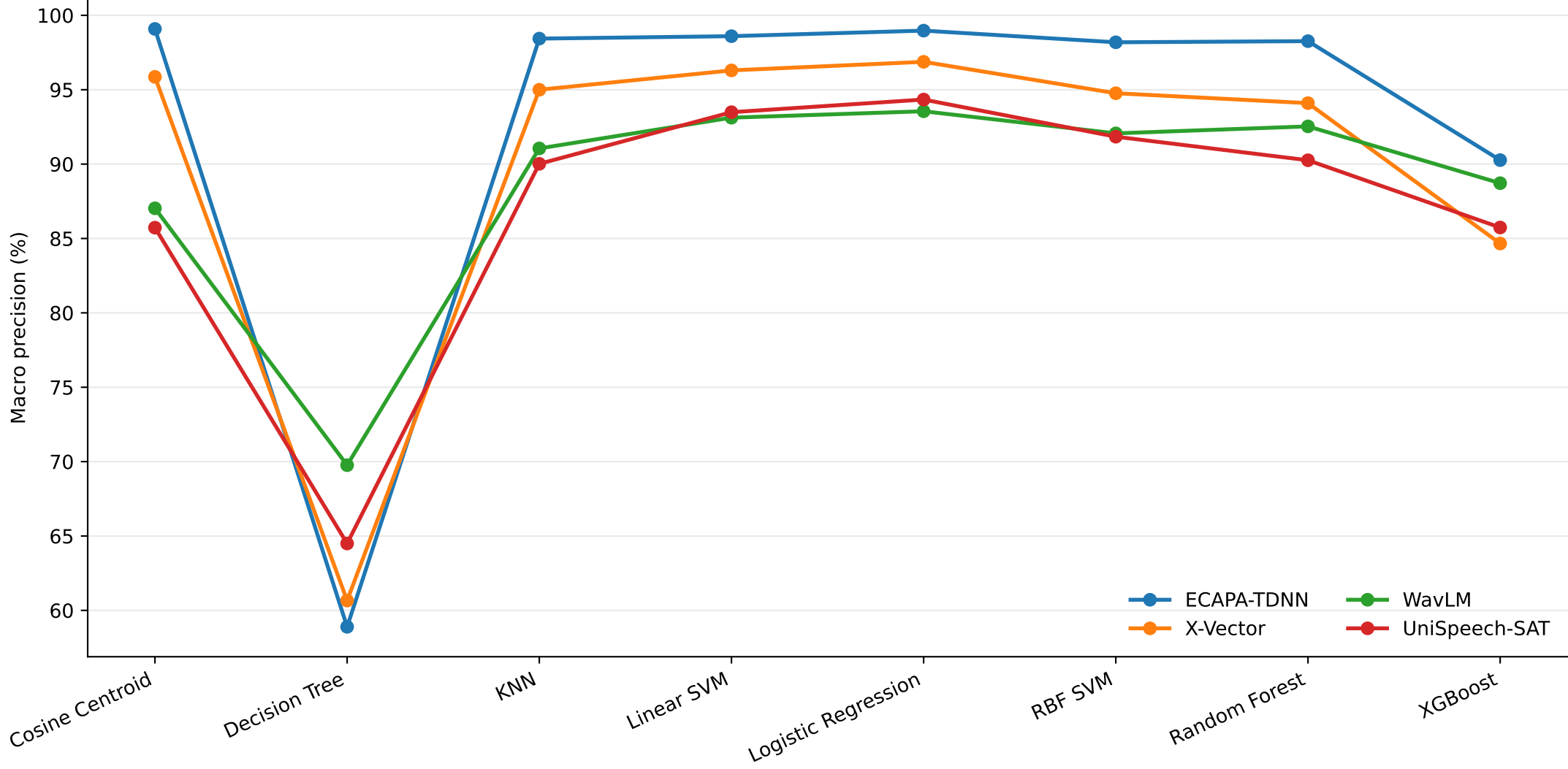
Macro precision by Embedding Model and Classifier
