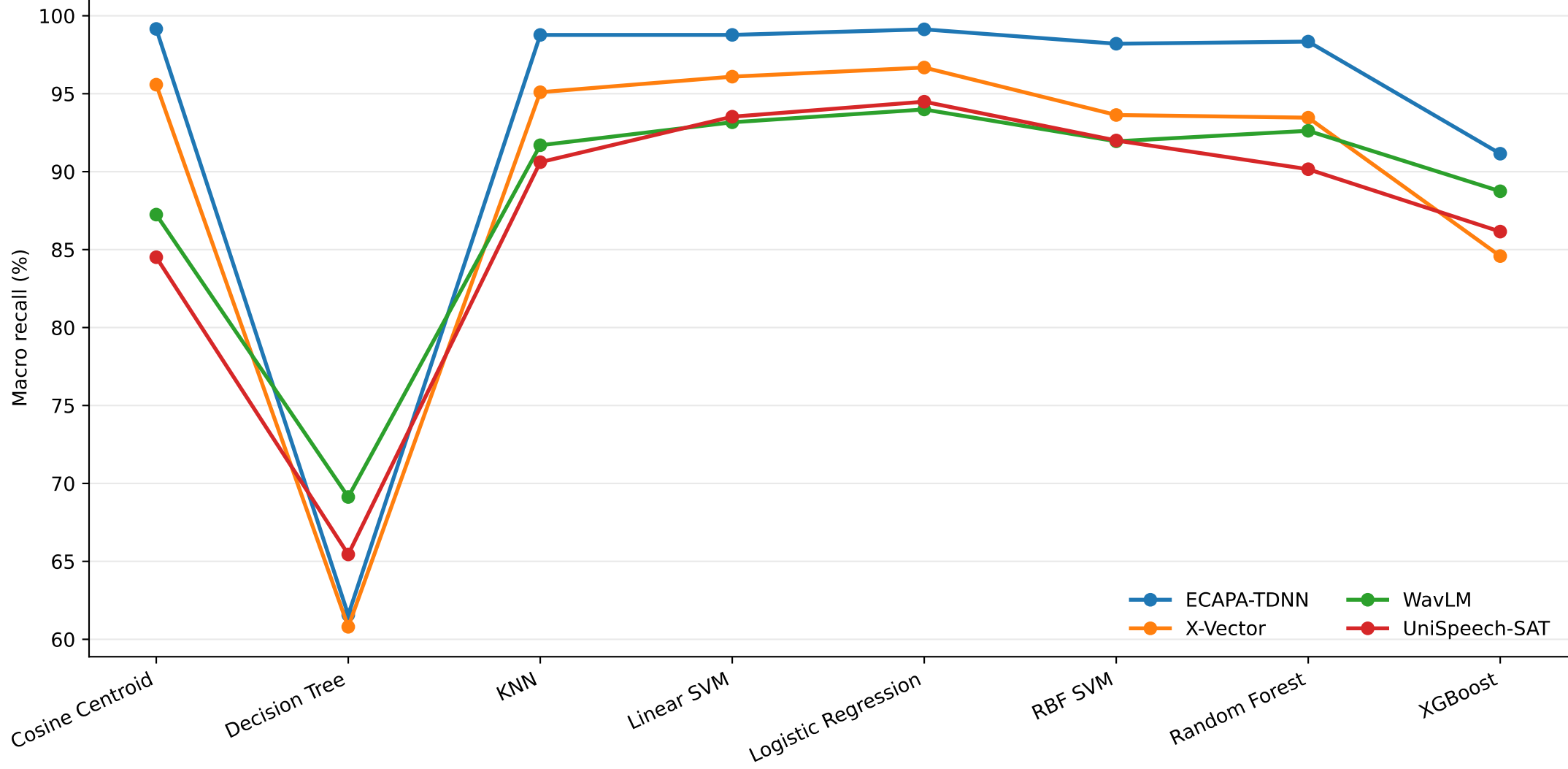
Macro recall by Embedding Model and Classifier
