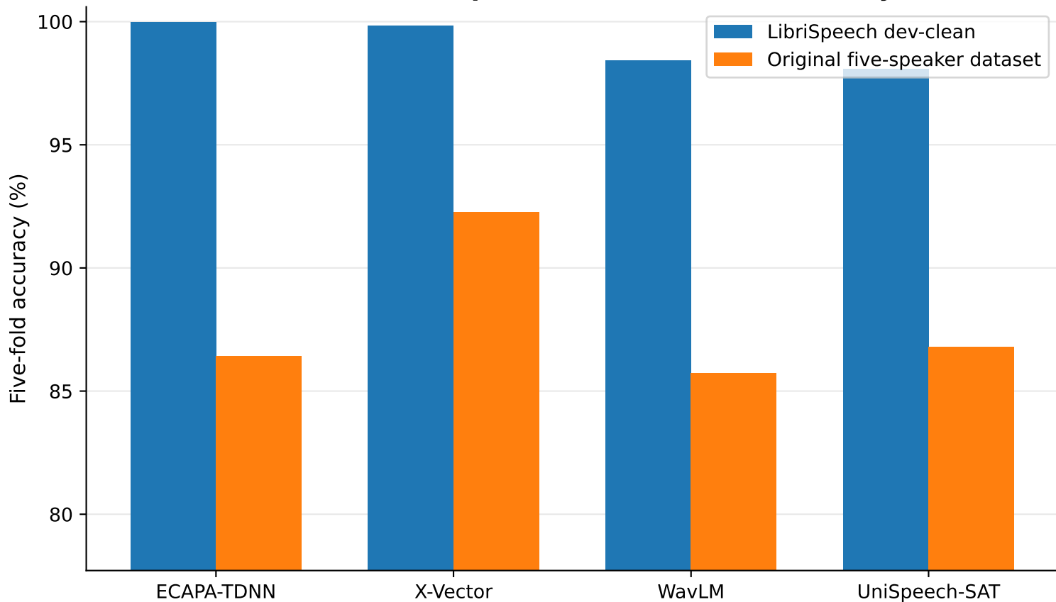
Cross-Dataset Speaker Identification Accuracy
