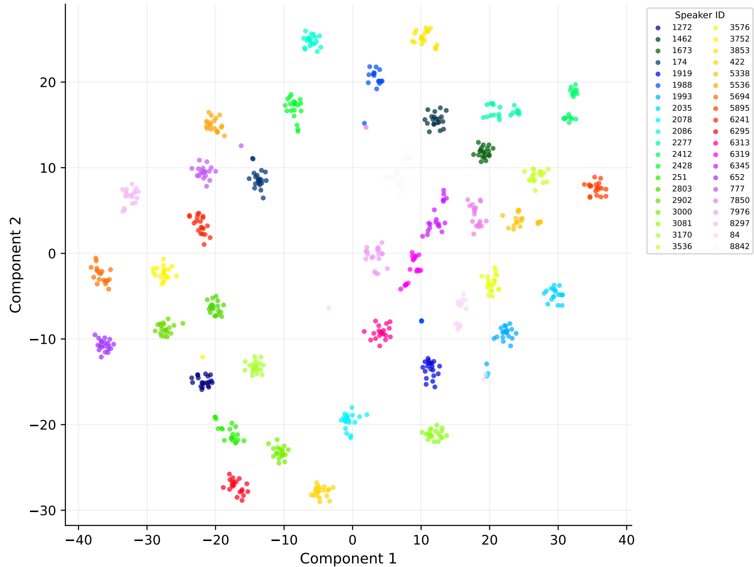
X-Vector — t-SNE Speaker Embeddings
