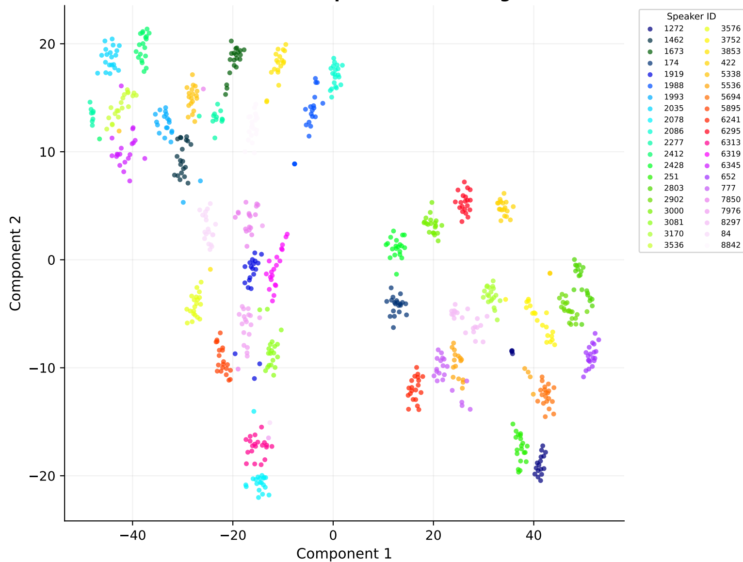
WavLM — t-SNE Speaker Embeddings
