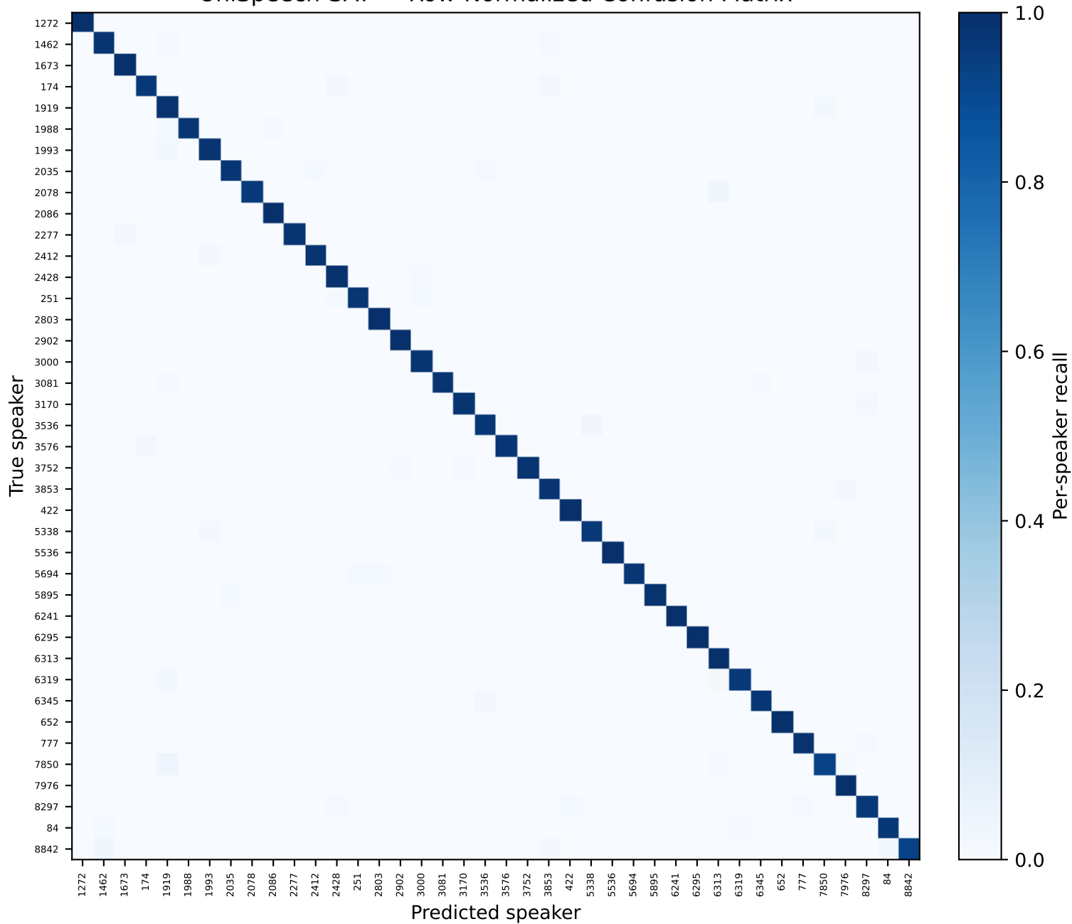
UniSpeech-SAT — Row-Normalized Confusion Matrix
