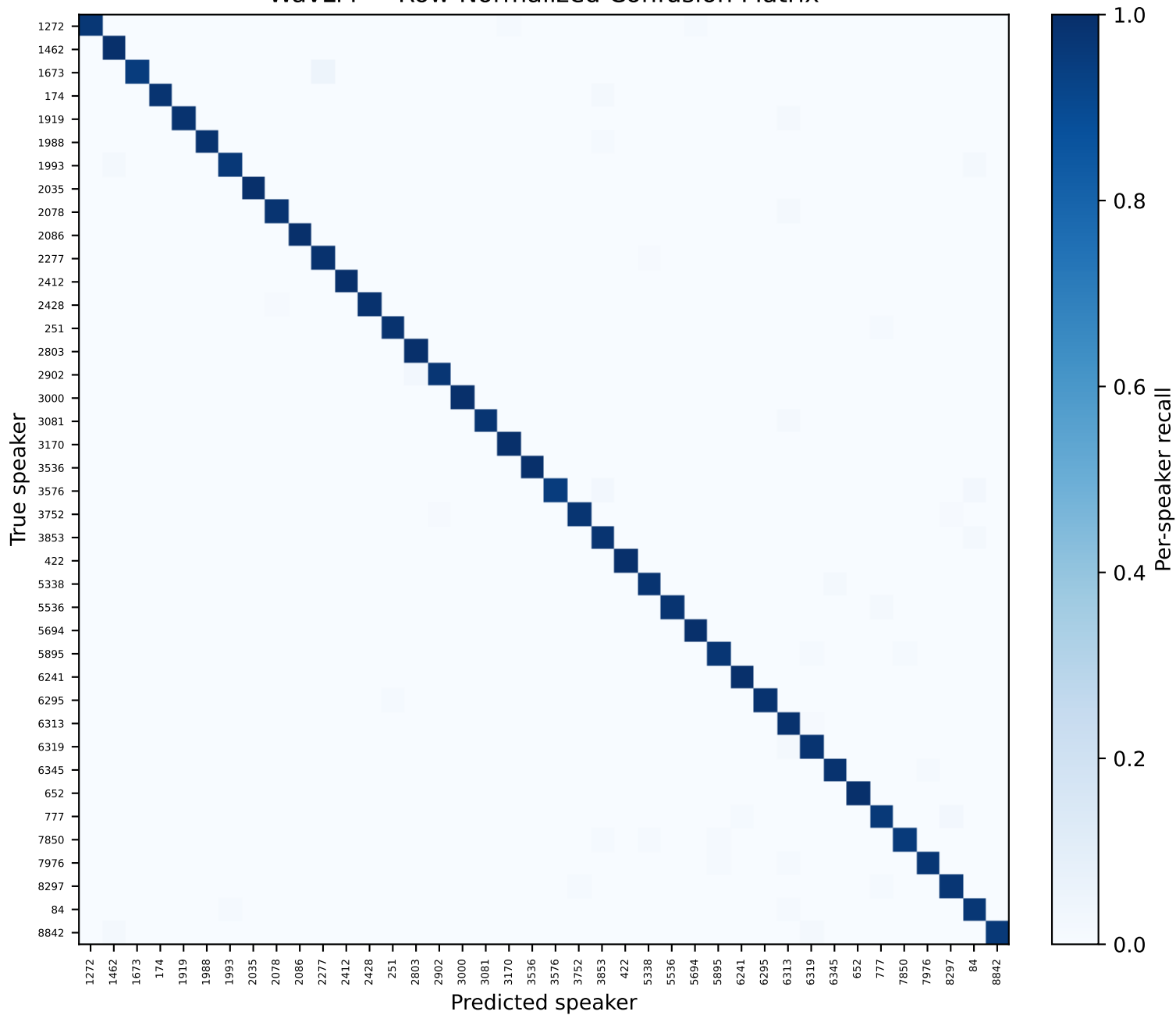
WavLM — Row-Normalized Confusion Matrix
