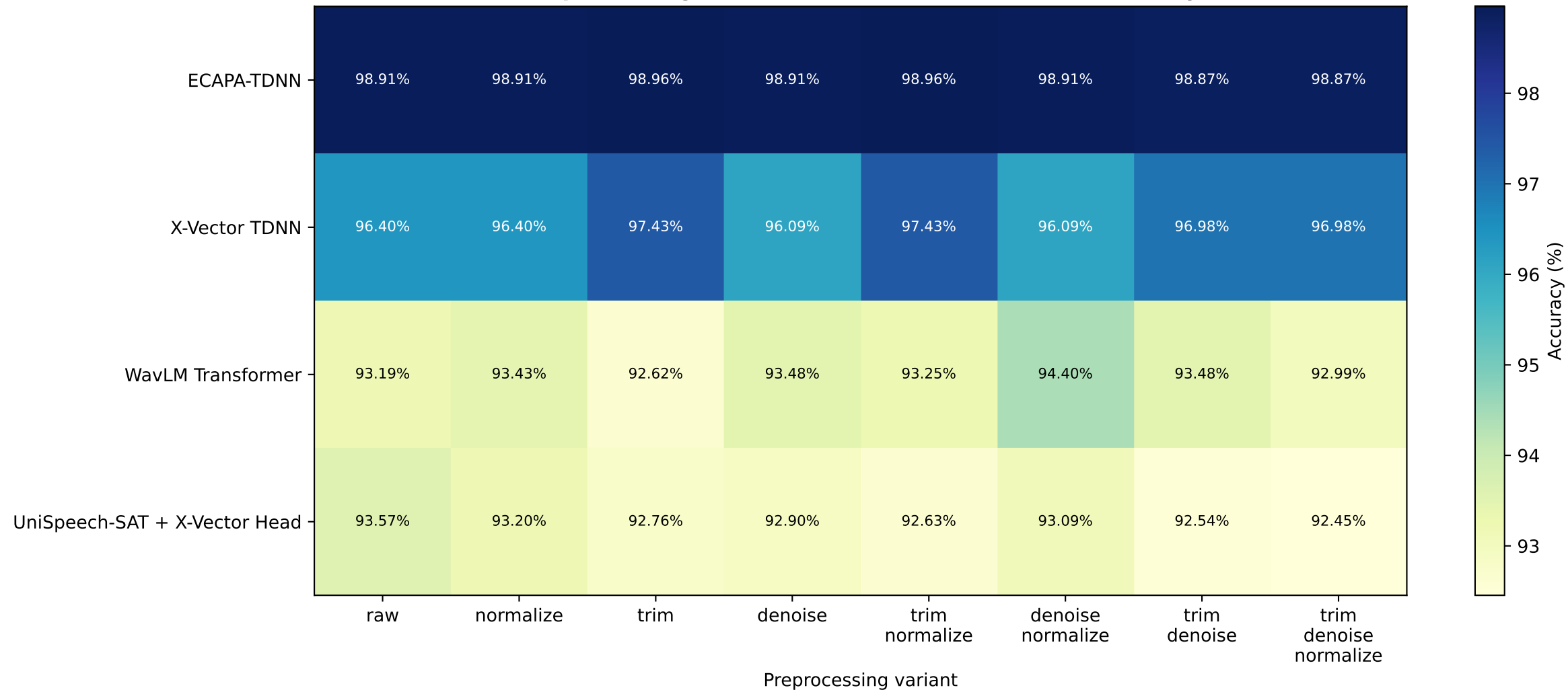
Preprocessing ablation: mean strict outer-fold accuracy
