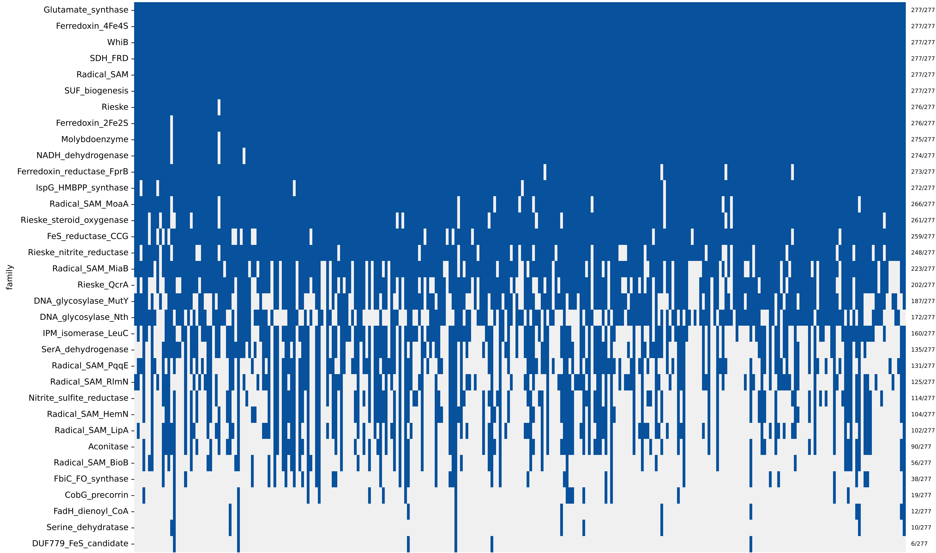
Fe-S family presence/absence (corrected)
