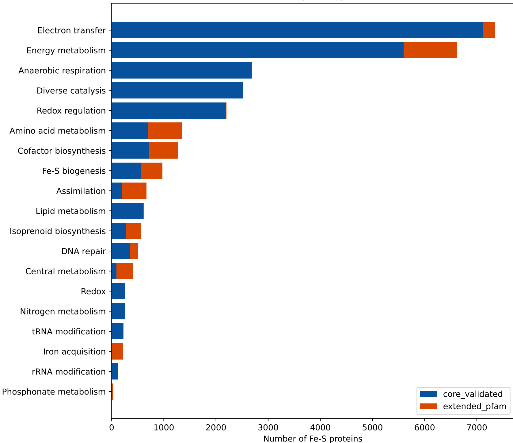
Fe-S functional categories by confidence tier
