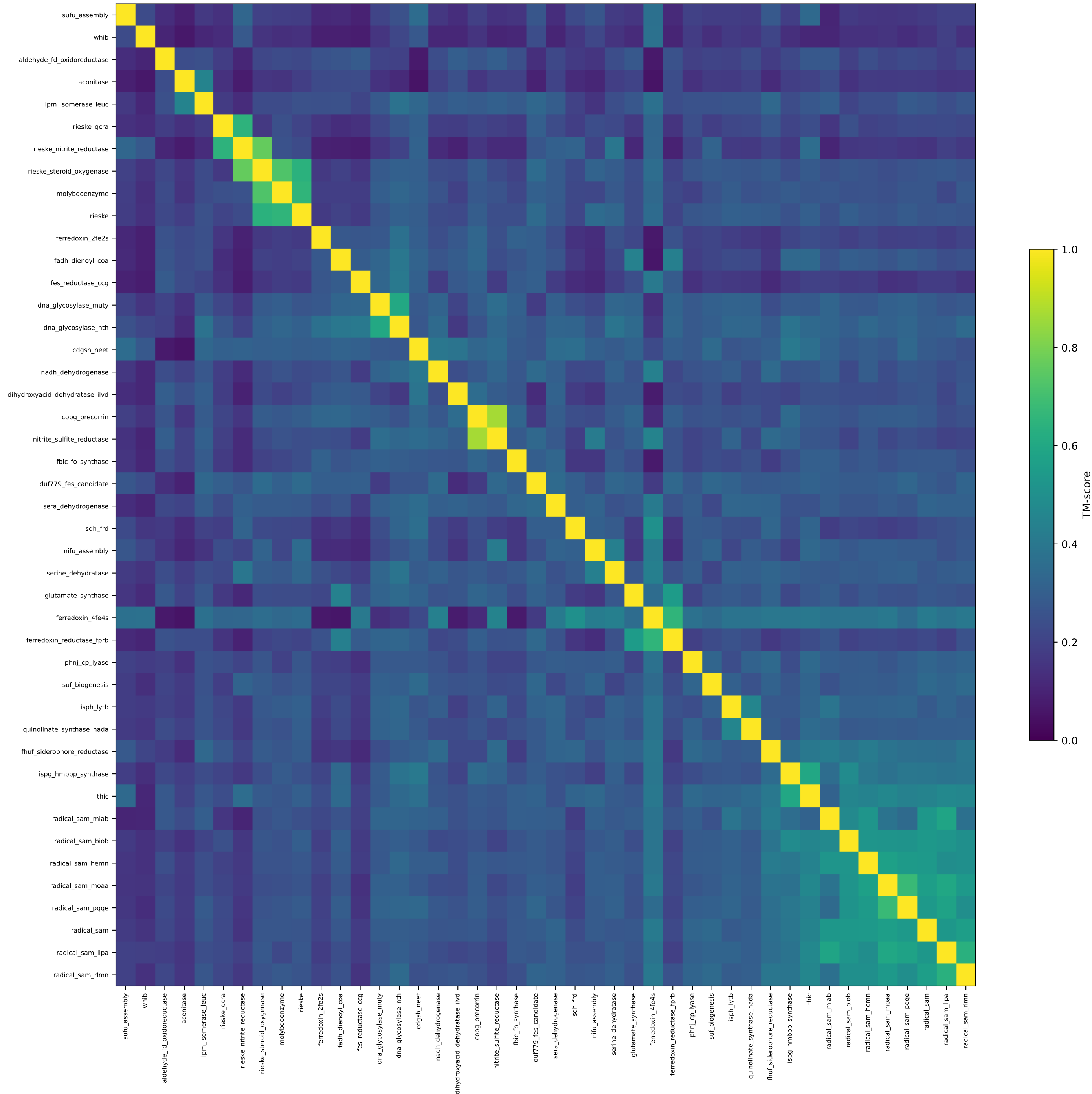
All-vs-all structural similarity of Fe-S family representatives (TM-align)
